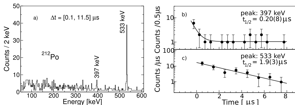
Fig. 2. (a) Delayed \gamma -ray spectrum of ^{212}\text{Po} , showing the two lines assigned to the depopulation of the states above the ( 18^+ ) isomer of this isotope. The spectrum has been produced selecting a time window of \Delta t = [0.1, 11.5] \mu\text{s} after the implantation. Both lines attributed to ^{212}\text{Po} present an exponential time distribution, displayed in panel b) for the 397 keV line (where also a constant background term is added) and in panel c) for the 533 keV line, along with their estimated half-lives.
