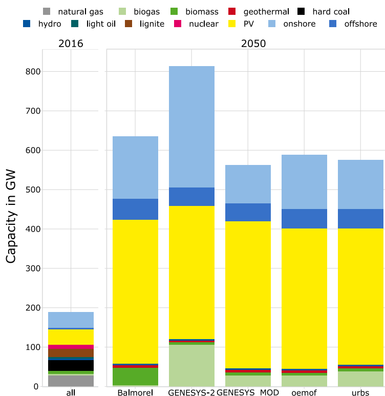
Fig. 1. Capacity results across frameworks (fixed for 2016, optimized for 2050).
