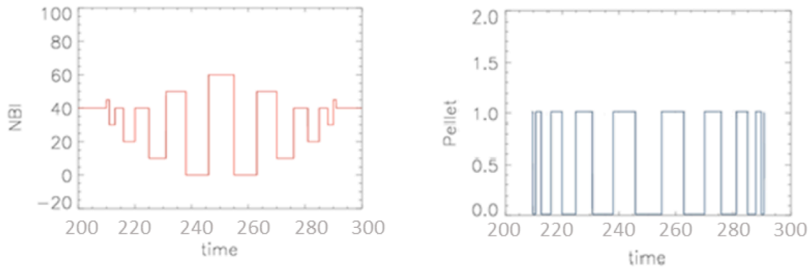
Fig. 7. Use of NBI (MW) and pellet injection (here 0 – 1 indicates injection off and on, respectively) to counteract to the W-flake event in Fig. 4–6. The pellet size, as discussed in the next section, amounts to 2 \cdot 10^{21} particles.
