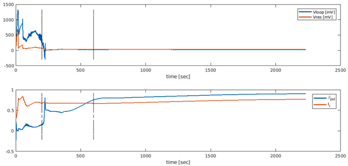
Fig. 2. Loop voltage (top), \beta_{pol} and l_i (bottom) for the ramp-up case shown in Fig. 1. In the top panel, the total loop voltage and its resistive fraction are shown. Black vertical lines identify the end of the current ramp (200 s) and the end of the density ramp (600 s).
