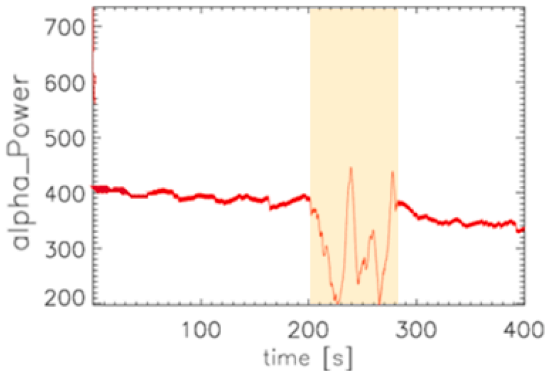
Fig. 6. Evolution of fusion \alpha -power when a W flake of 1 mg is introduced (at t = 200 s). Power is expressed in MW. After large oscillations, the discharge has been successfully recovered. The occurrence of the instability has been highlighted with a light yellow shading (For interpretation of the references to color in this figure legend, the reader is referred to the web version of this article.).
