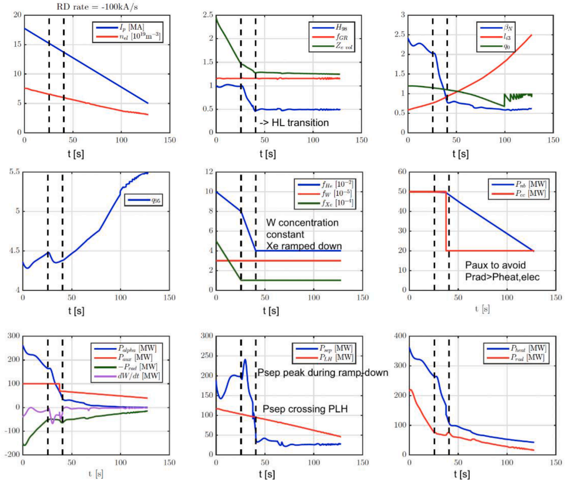
Fig. 4. Evolution of main plasma quantities during a ramp-down case at -100 kA/s produced with RAPTOR. According to the definitions introduced in Fig. 3, this is an early HL, cold L case, i.e. the best case scenario. This ramp trajectory is marginally unstable (in terms of position control) if the criterion 1.25l_i is adopted – see Fig. 3.
