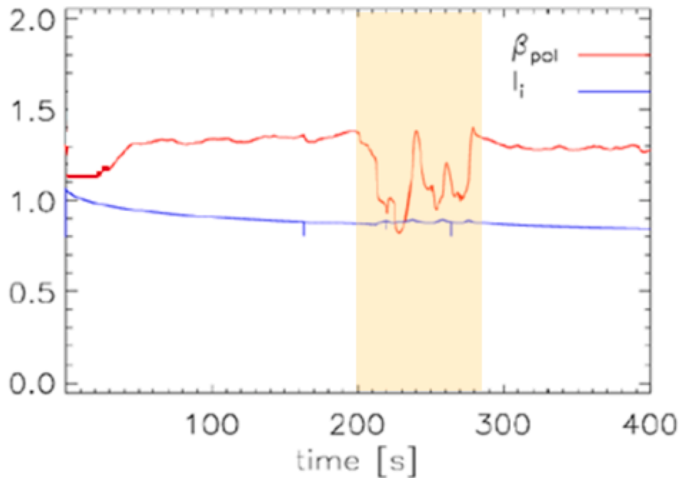
Fig. 8. Evolution of \beta_{pol} and I_i when a W flake of 1mg is introduced (at t = 200 s). Oscillations are quite large but still recoverable by the position control system. The occurrence of the instability has been highlighted with a light yellow shading (For interpretation of the references to color in this figure legend, the reader is referred to the web version of this article.).
