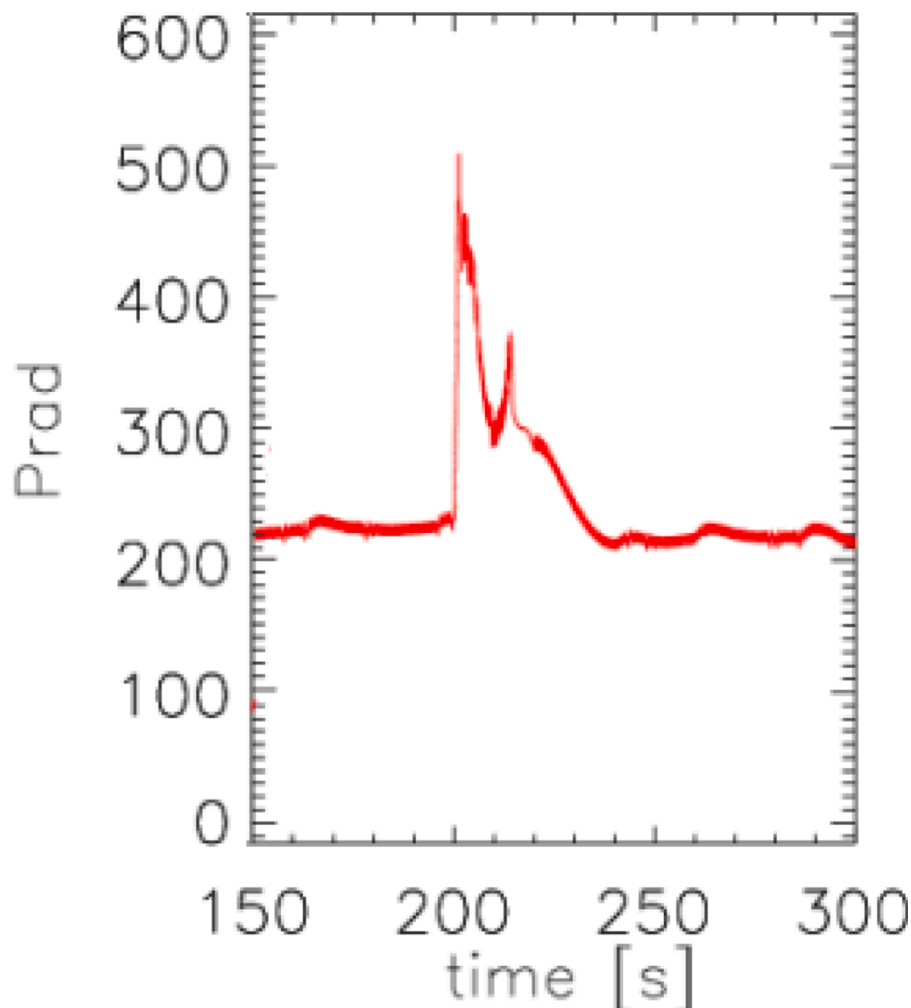
Fig. 5. Evolution of plasma line radiation when a W flake of 1 mg is introduced (at t = 200 s). Power is expressed in MW.
