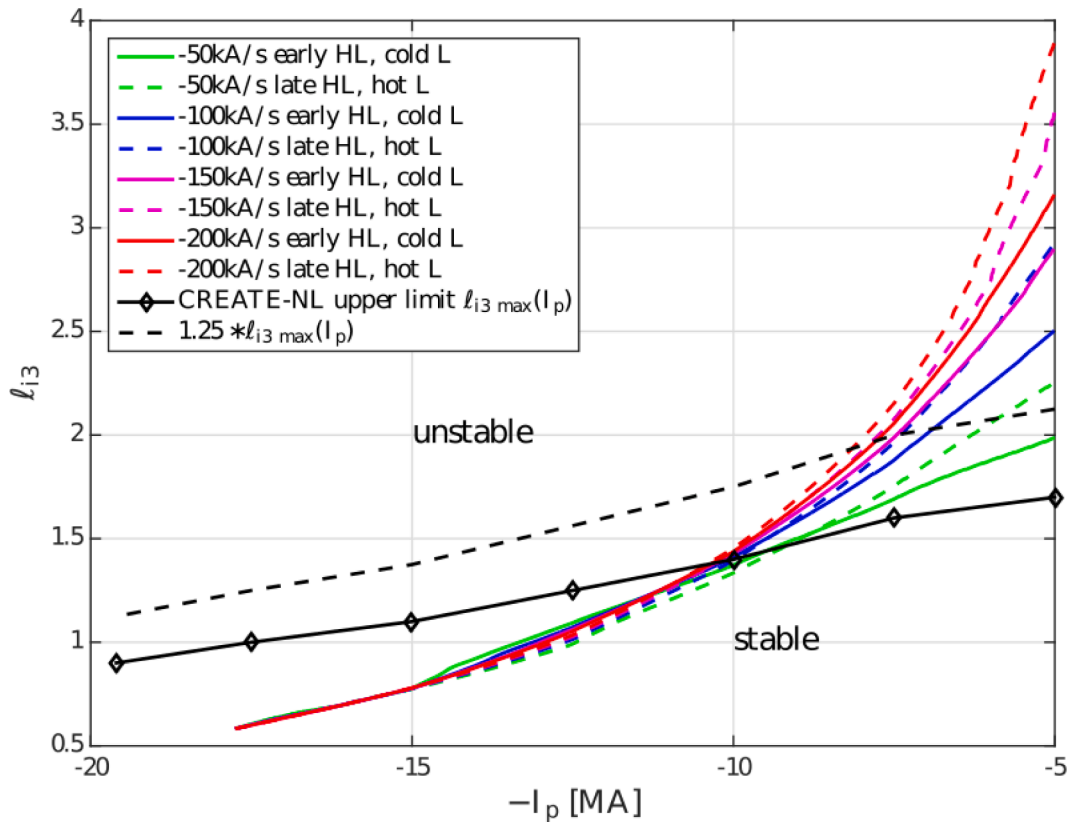
Fig. 3. Corresponding evolution of the internal inductance as a function of the plasma current during ramp-down phase. The definition of “hot”, “cold”, “early” and “late” is to be found in the main text. The black diamond line indicates the maximum allowable internal inductance compatible with the imposed magnetic equilibria, while the dashed line corresponds to the same value multiplied by 1.25 – i.e. allowing for some margin.
