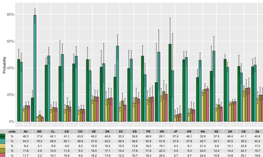
Fig. 10. Prediction scenario 2: high efficacy vaccine with three month wait but high risk of side effects vs low efficacy vaccine with immediate access and low risk of side effects (95% confidence intervals by bootstrapping from parameter distribution using asymptotic variance-covariance matrix).
