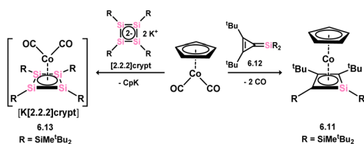
Scheme 47 Formation of cobalt complexes of the tetrasilacyclobutadiene-diide and silacyclobutadiene-diide ligands via differing routes.
