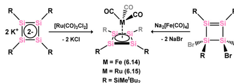
Scheme 48 Formation of ruthenium and iron complexes of the tetrasilacyclobutadiene-diide ligand.
