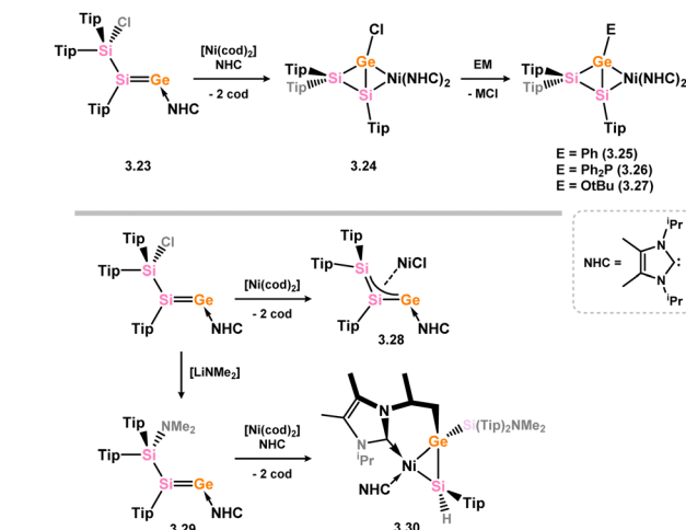
Scheme 23 Formation of a nickel(0) complex of a disilagerma-cyclopropene (above), and a closely related disilagerma-allyl complex of nickel(II).
