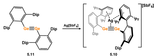
Scheme 40 Complexation of a digermine with silver(i).
