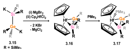
Scheme 21 Formation of a hafnium complex bearing a germsilene ligand.
