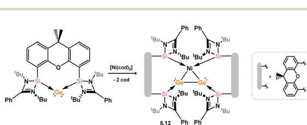
Scheme 41 Formation of a \text{Ge}_2 -Ni \pi -complex from a geryllone.
