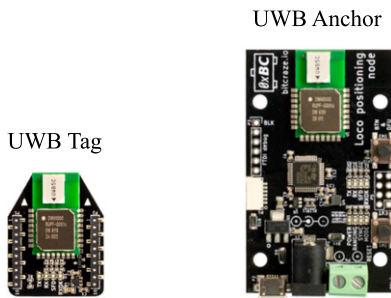
Figure 2. The Loco Positioning System anchor and tag from Bitcraze, based on Decawave’s DWM1000 UWB modules, are used for the data collection.
