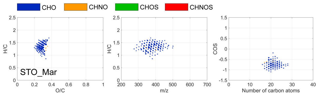
Fig. 6 van Krevelen diagrams (left panel), mass edited H/C ratios (middle panel) and average oxidation state of carbon plots (right panel) of the molecular compositions that decreased in relative abundance by more than 50% after the addition of monochloramine in STO in March. Point size reflect relative mass peak intensity in a sample.
