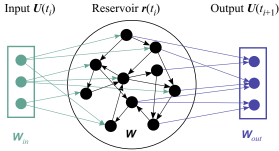
Figure 3. Schematic representation of an echo state network.
