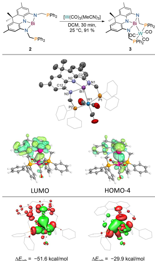
Fig. 4 Synthesis of 3 upon addition of [W(CO) 3 (MeCN) 3 ] to 2 (top); molecular structure of 3 in the solid state obtained via SCXRD, ellipsoids at 50% probability level; H atoms are omitted for clarity, one molecule of the asymmetric unit shown; and selected computed frontier molecular orbitals (middle, Me groups of the acridane ligand truncated to H); selected donor (red)/acceptor (green) orbital pairs derived via energy decomposition analysis showcasing the ligand's redox activity as well as the ambiphilic bonding between tungsten and bismuth (bottom).
