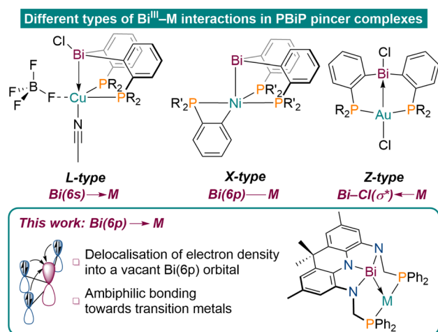
Fig. 1 Representative examples of established bonding modes of Bi(III) R 3 derived transition metal pincer complexes (top, R = Ph, R' = 'Pr); 7–9,12 our results on realizing ambiphilic Bi(6p)–M bonding (bottom).
