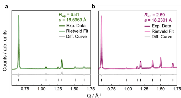
Fig. 2 Rietveld refinements against high-resolution PXRD pattern at ambient pressure of \text{Fe}(\text{ta})_2 (a) in green and \text{Fe}(\text{cta})_2 (b) in purple. Experimental data is shown as dark line, the calculated data from Rietveld refinement as light line, and the difference curve (fit – data) as grey line. Reflection positions are shown as black vertical tick marks. Rietveld fit of \text{Fe}(\text{mta})_2 is given in the ESI† (Fig. S20).
