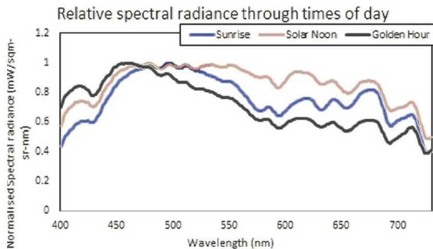
Fig. 4 Normalised relative SPD at Sunrise, Solar Noon and Golden Hour (typical data for the 3 days)
