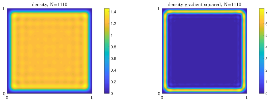
Figure 2.1: Density (left) and density gradient squared (right) of the free electron gas with 1110 electrons in a three-dimensional box with zero boundary conditions. The picture shows a two-dimensional cross-section through the center of the box, and the number of electrons per unit volume was normalized to 1. The density gradients of order 1 near the boundary persist in the thermodynamic limit.
