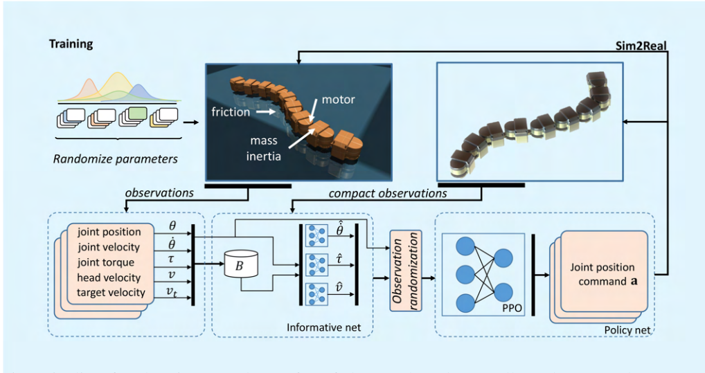
Fig. 2: The training pipeline for the sim-to-real transfer of the NN-based controller. There are three steps in this pipeline. First, the physical parameters are randomized in each episode during training. Second, the observation space is used to train an informative neural network to predict the observations that can not acquired directly from real-world environments. Third, the randomized observations are fed to the NN-based controller, which is trained using PPO algorithm.
