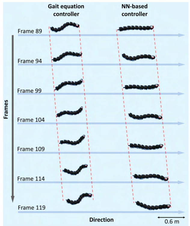
Fig. 7: The montages of the snake-like robot performing slithering gait at 0.15 m/s, controlled with the NN-based controller and the gait equation controller. The video is recorded at 25 frames per second.
