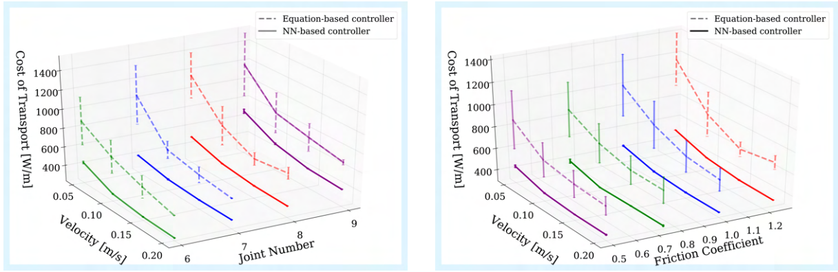
(a) The gaits are generated with robots with different designs (number of the body module).
