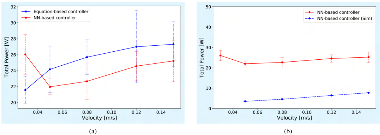
Fig. 8: (a) Real-world power comparison of the slithering gaits from the gait equation controller and the NN-based controller. The target velocities are [0.05, 0.10, 0.15, 0.2, 0.25] m/s. The actual velocities are [0.03, 0.05, 0.08, 0.12, 0.15] m/s, approximately. The solid points represent the averaged power over 10 s and the error bars depict the standard deviation. Note the standard deviation is calculated based on the data over the duration of the experiment (10 s). (b) Power comparison of the NN-based controller in the simulation and the real world. In simulation, the NN-based controller cannot achieve a gait that is 0.03 m/s.
