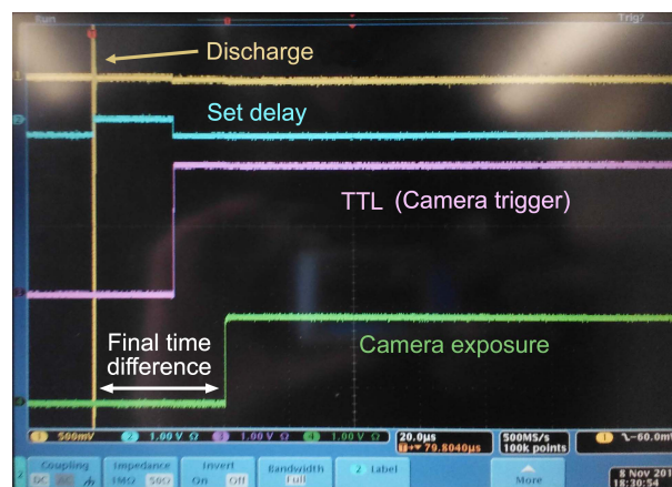
Figure 5. The signals used for the triggering of the camera. Yellow: The electrical signal induced by the primary discharge measured at the anode. Blue: Adjustable delay to control the time difference between camera exposure and discharge. Purple: The trigger sent to the camera. Green: Gate from the camera showing the exposure of the sensor.
