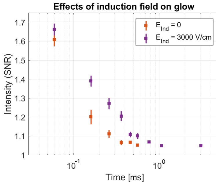
Figure 7. The observed glow evolution for Ar-CO 2 (90-10) using Retiga CCD camera. The measurements are conducted with 0 and 3000 V/cm applied induction fields, with the latter being close to the required field strength to produce propagations.
