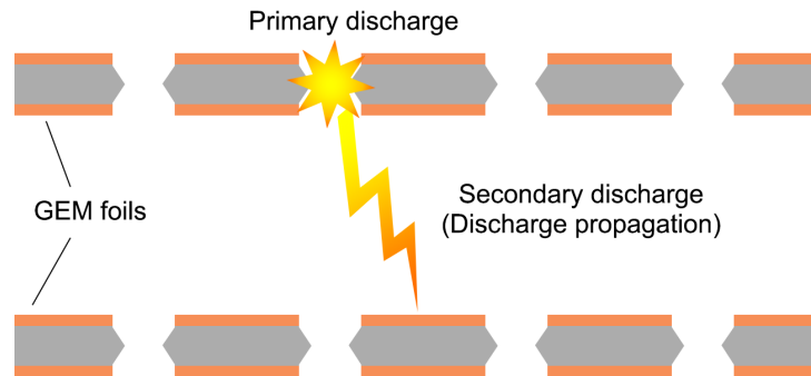
Figure 1. Schematic of the two types of GEM discharges.
