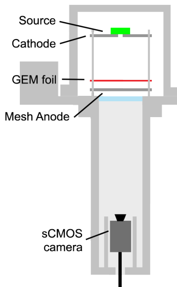
Figure 2. Sketch of the detector setup.
