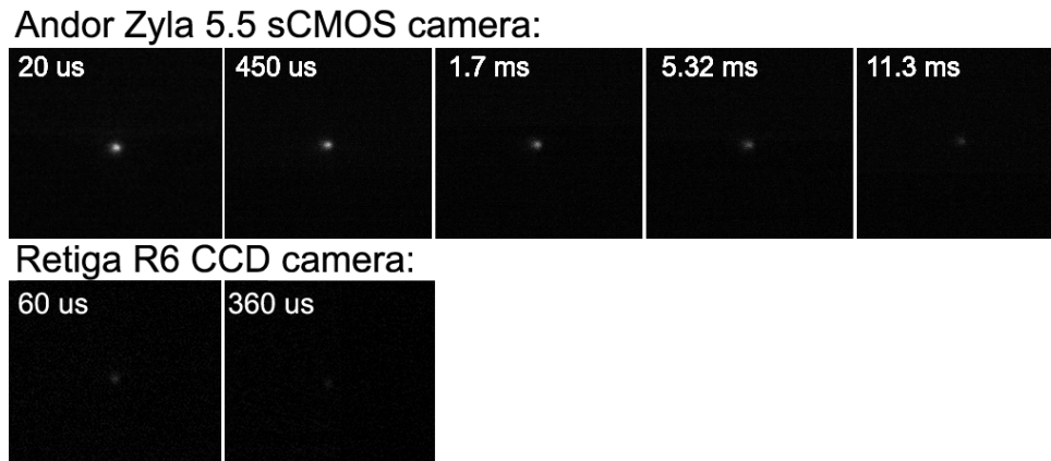
Figure 6. The observed time evolution of the glow after a primary discharge compared between two use scientific cameras. Given time information is for the initial signal peak from the primary discharge being in time 0.
