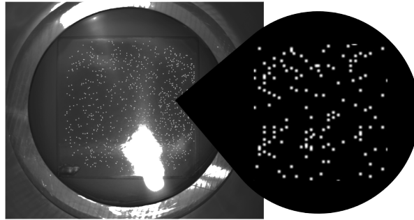
Figure 4. Combined image of multiple primary discharges with a close up on a section of the foil. Discharges in neighbouring holes can be distinguished and the hexagonal hole pattern can be recognised.
