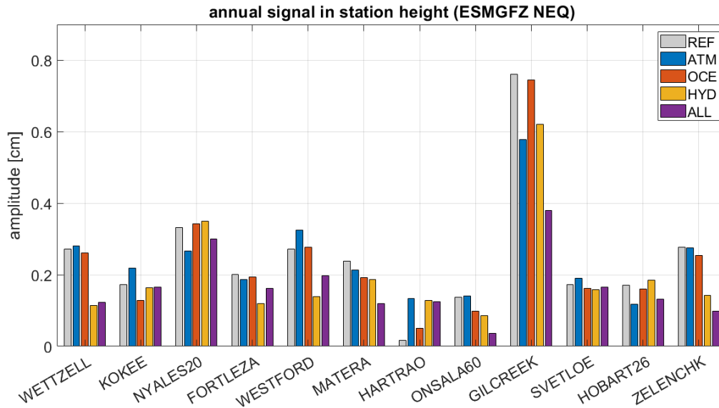
Fig. 1 We analysed more than 4,000 sessions between 1984 and 2017. For each of them, 5 different setups were used: no non-tidal loading (REF), non-tidal atmospheric loading only (ATM), non-tidal oceanic loading only (OCE), hydrological loading only (HYD), all non-tidal loading types at once (ALL). Here, we compare the amplitudes of the annual signal in the time series of station heights for all distinct setups, and observe that the signals are often reduced when hydrological loading is applied (HYD, ALL). The non-tidal loading data has been taken from the Earth System Modelling group of the Deutsches GeoForschungsZentrum and applied at the normal equation level.
