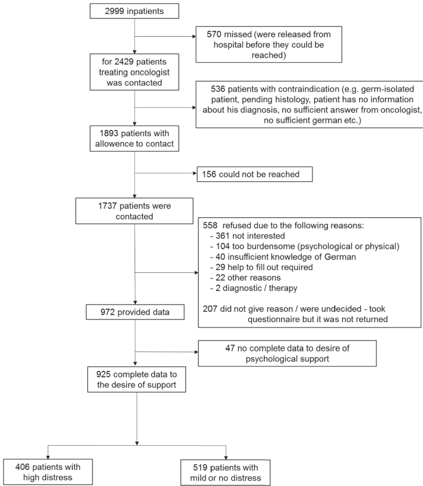
Study flowchart
