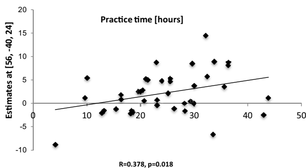
Figure 3. (A) The results of group-by-time analysis mapped onto Conte69 atlas via Connectome Workbench using trilinear interpolation. (B) Parameter estimates extracted from the peak [56, -40, 24], Brodmann area 40, using second-level 1-sample t tests for each group and condition using the extinguished vs. conditioned stimulus never paired with the shock (CS+E vs. CS-) contrasts. Compared with the control intervention, the mindfulness-based stress reduction (MBSR) intervention was associated with the higher engagement of a cluster in the right supramarginal gyrus (rSMG)/posterior parietal cortex. (C) Neural activity (parameter estimates of blood oxygen level-dependent signal extracted from the peak following MBSR intervention) correlate with total amount of home meditation practice during the MBSR intervention. (D) Changes in hippocampal functional connectivity during extinction recall following MBSR. FWEc, cluster level familywise error; MNI, Montreal Neurological Institute; rSMG, right supramarginal gyrus.
