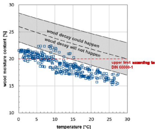
Figure 7: Temperature-dependent boundary for the assessment of the potential wood decay
