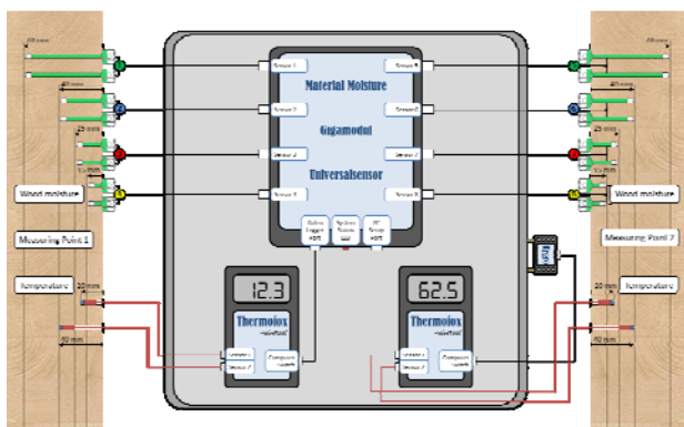
Figure 2: Schematic illustration of the measuring system
