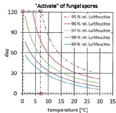
Figure 5: wood-decaying model of Viitanen [8] – phase I: "Activate" of fungal spores
