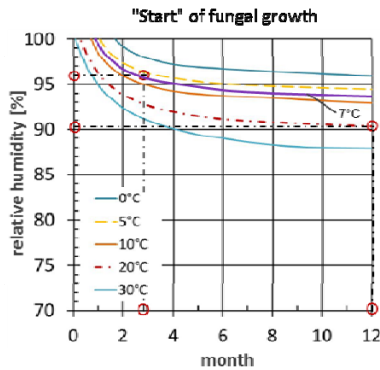
Figure 6: wood-decaying model of Viitanen [8] – phase II: “Start” of fungal growth
