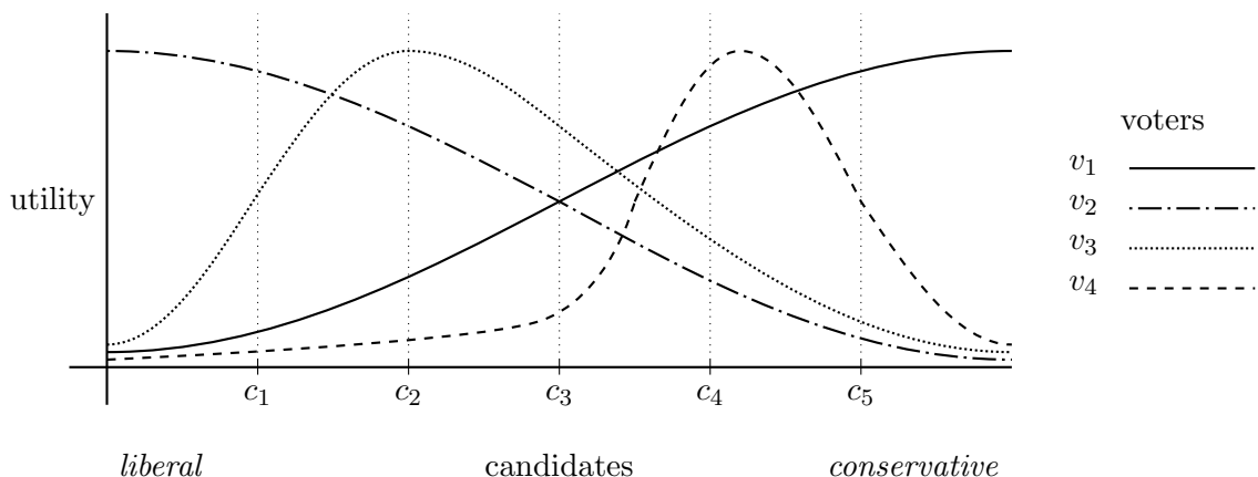
Figure 1: Example of a single-peaked electorate of four voters, with their utility functions shown.
