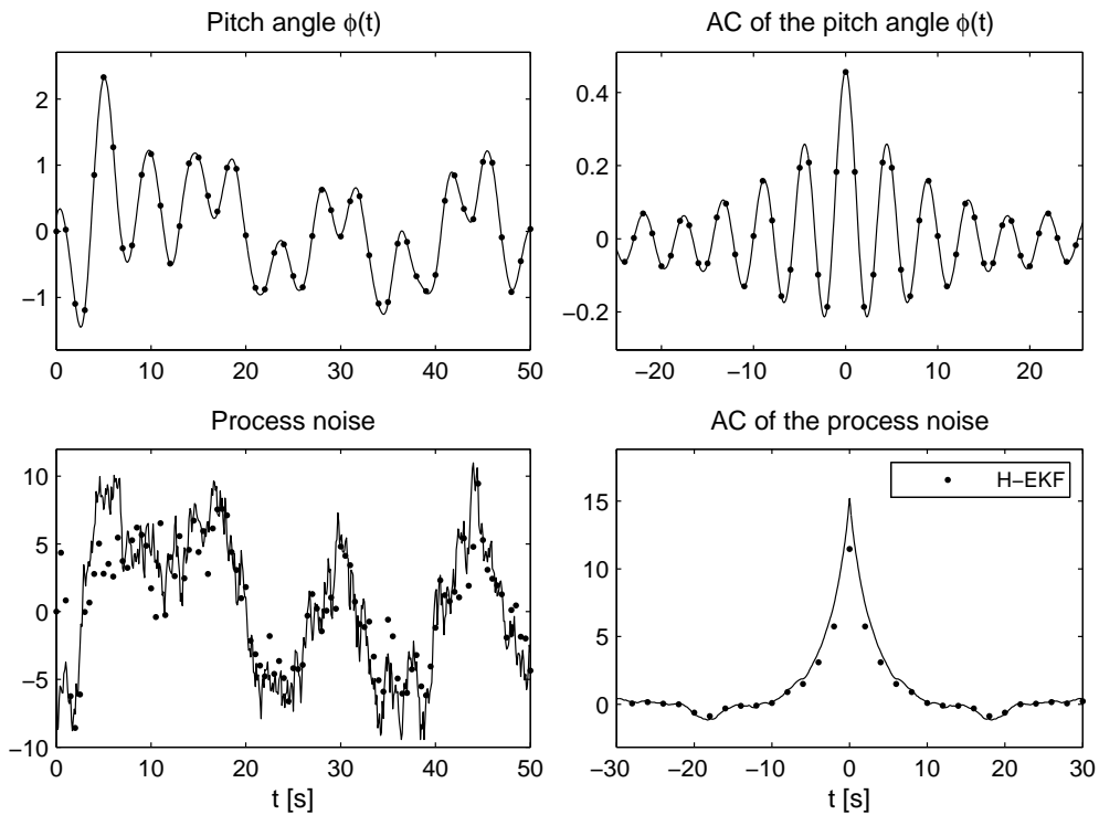
(b) Top: Evaluation of the pitch angle \phi(t) [rad] and AC function R_\phi(t) [rad 2 ] for \omega = \sqrt{2} [rad/s], D = 0.05 [-], Bottom: Actual process noise (line) and estimated input by the H-fractional EKF (points) and corresponding AC function R_F [N 2 ]
