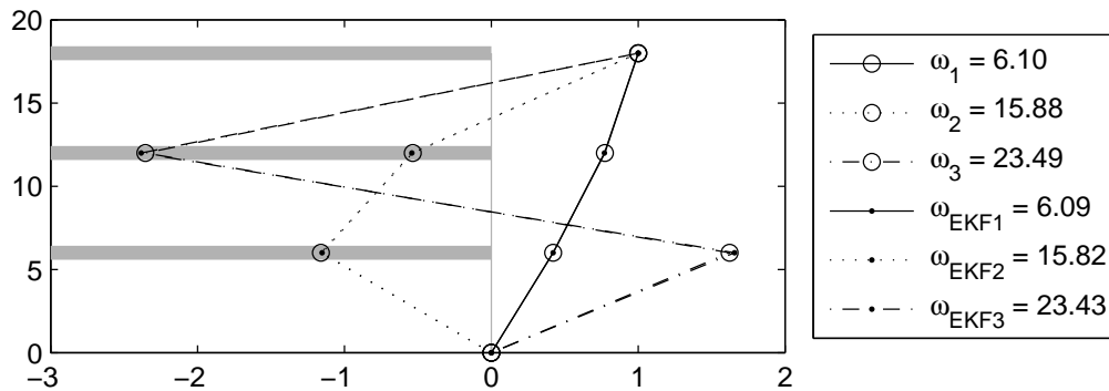
Figure 6.11: Comparison of the exact and estimated eigenfrequencies and modes for the case \sigma_p^2 = 1 \times 10^6 and a measurement noise of 10 [%]
