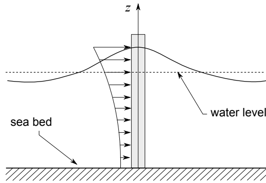
Figure 2.18: Distribution of the wave force [Li and Chen 2009, p. 67]
