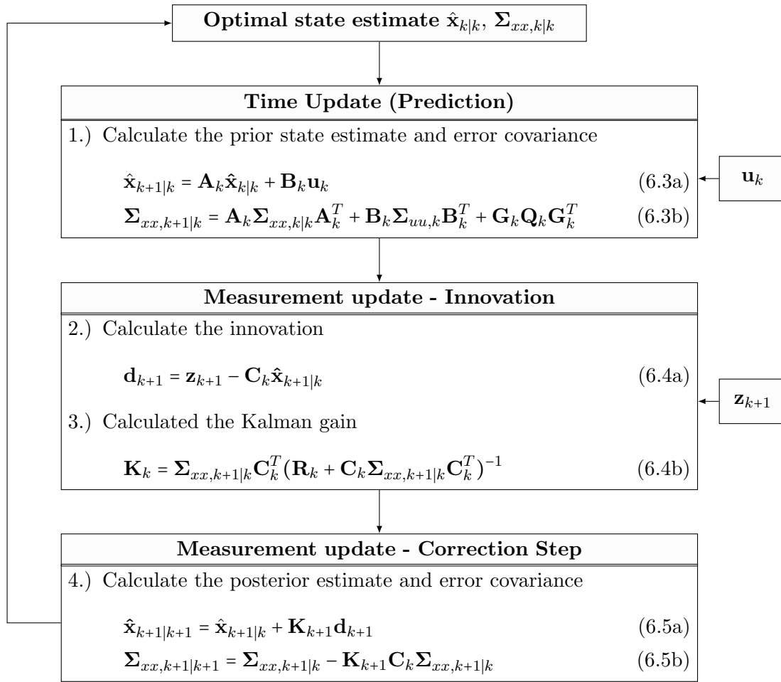
Figure 6.2: Kalman filter algorithm
