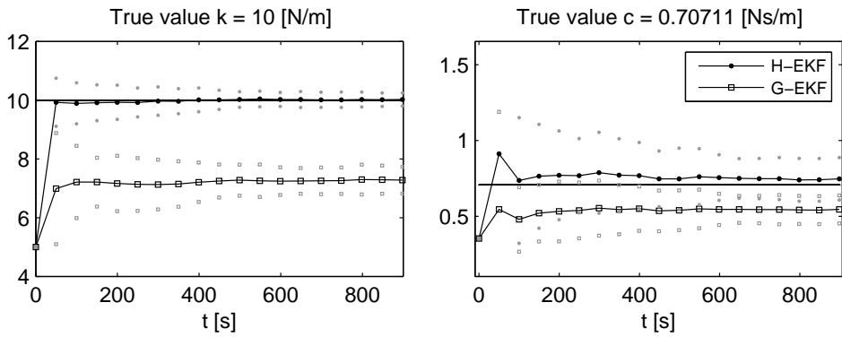
(a) Estimation of the stiffness k [N/m] and damping constant c [Ns/m] of the by means of H-fractional EKF (points) and the Gaussian EKF (squares). The dotted lines represent the corresponding 90 % confidence intervals.
