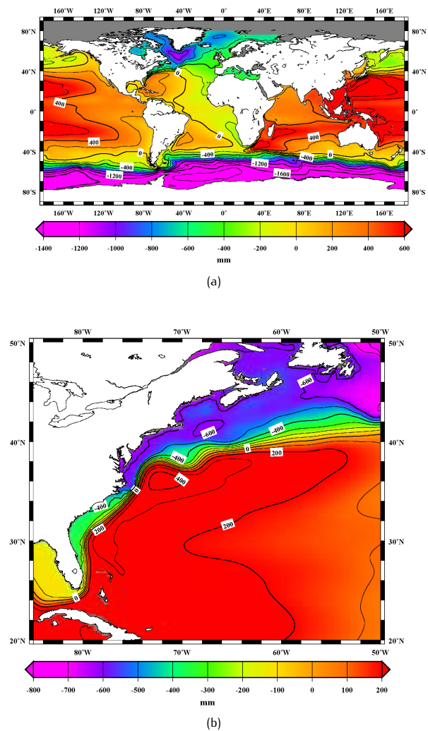
Figure 1. (a) The global Mean Dynamic Topography (MDT) for the period 1993-2002 from the 'coarse grid' Liverpool-MIT ocean model. Contours every 200 mm, (b) the MDT from the 'fine grid' version of the same model focussing on the western North Atlantic. Contours every 100 mm.
