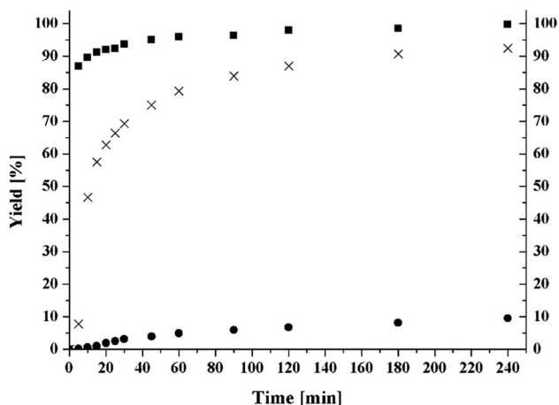
Fig. 3 Kinetics of the tricarbonyl complexes 1 [CpMo(CO) 3 Cl] (■), 2 [CpMo(CO) 3 CH 3 ] (X) and 3 [CpMo(CO) 3 CF 3 ] (●). Catalyst:cyclooctene: tert -butylhydroperoxide (TBHP); ratio: (0.0025 : 1 : 1.2); T = 25 °C.
