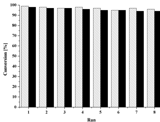
Fig. 4 Recycling experiments using compound 1 (dashed line) and compound 2 (black). Reaction conditions: 1 mmol of cis -cyclooctene, 2 mmol of TBHP in n -decane, 0.5 mol% catalyst, 55 °C, 0.5 mL of ionic liquid, 24 h reaction time. The yield was determined via GC (for details see the experimental section).
