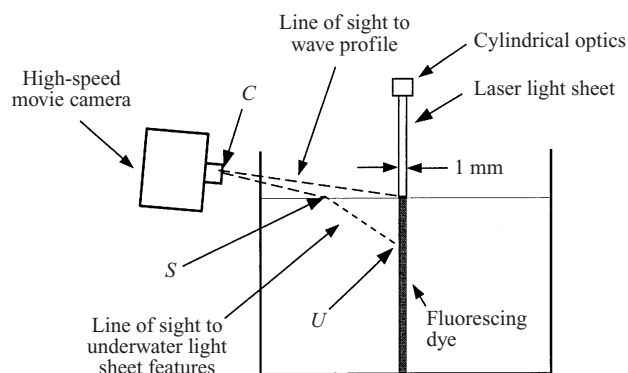
FIGURE 5. Schematic showing end view of tank with light sheet and fluorescing dye.
