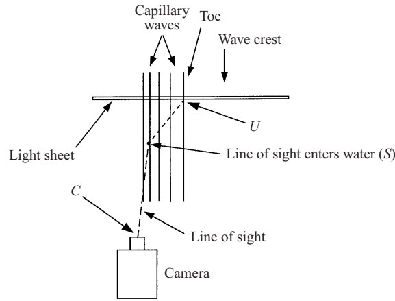
FIGURE 12. Schematic showing plan view of wave with camera, laser light sheet and line of sight to underwater features within the light sheet. See also figure 5.
