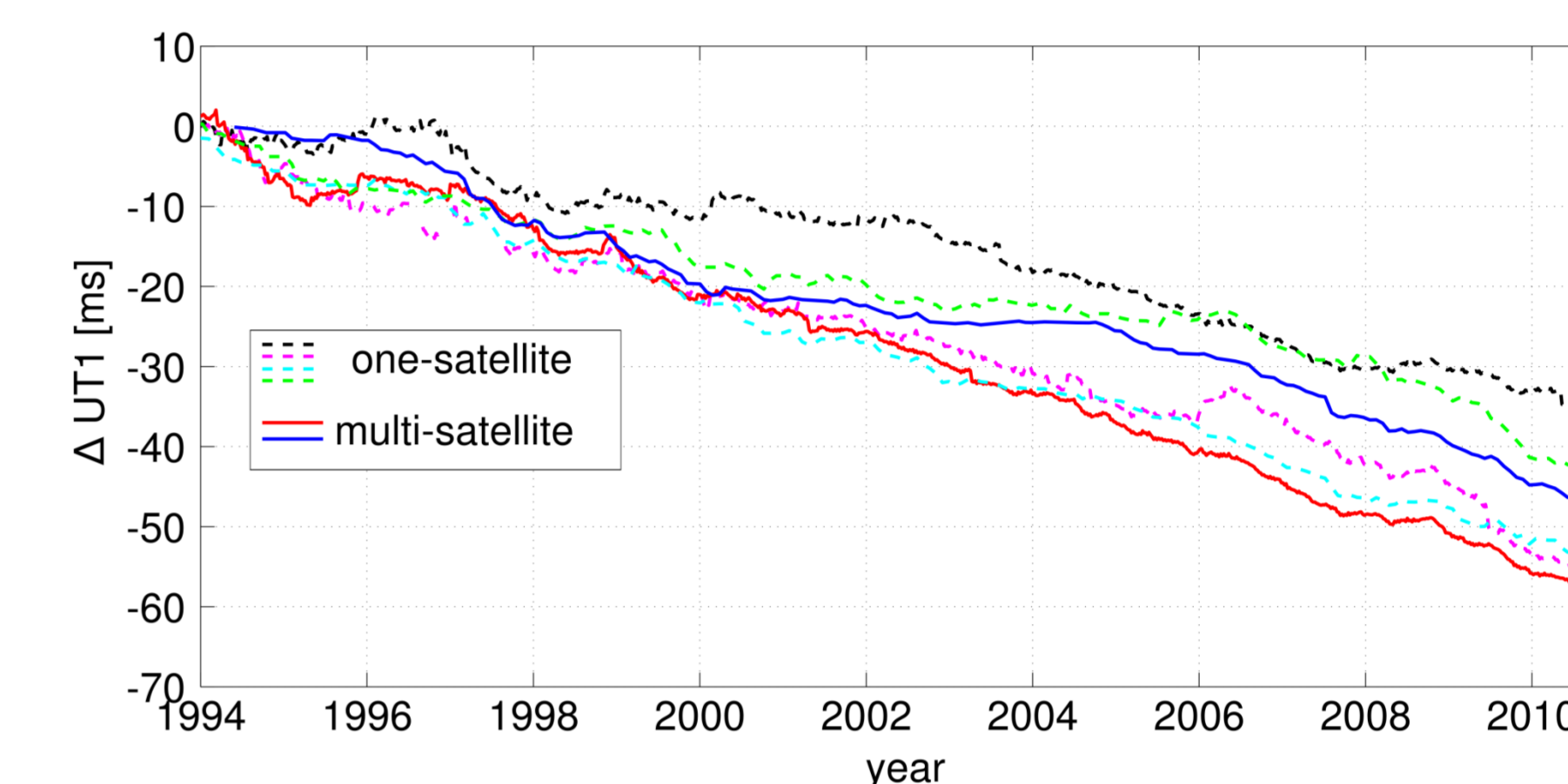
Fig. 5: Accumulated differences of UT1 w.r.t. IERS 08 C04 over a time span of 16.5 years. All solutions of the second iteration show a systematic drift in the order of -2.8 to -3.9 ms/y (Tab. 3).
