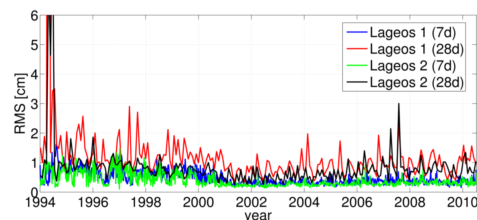
Fig. 1: Fits of the 7-day/28-day orbits of LAGEOS 1 and 2. Only observations from official core stations of the International Laser Ranging Service (ILRS) are considered.
