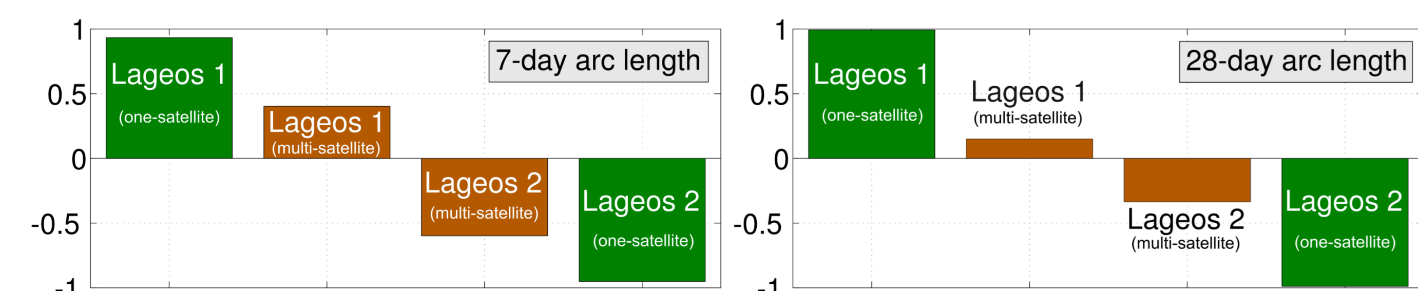
Fig. 2: Mean correlations of C_{20} and \Omega for one-satellite solutions (green-coloured) and multi-satellite solutions (orange-coloured). In the left part of Fig. 2 the mean correlations of solutions with an arc length of 7 days are shown, whereas the right part illustrates the same situation for a 28-day arc.
