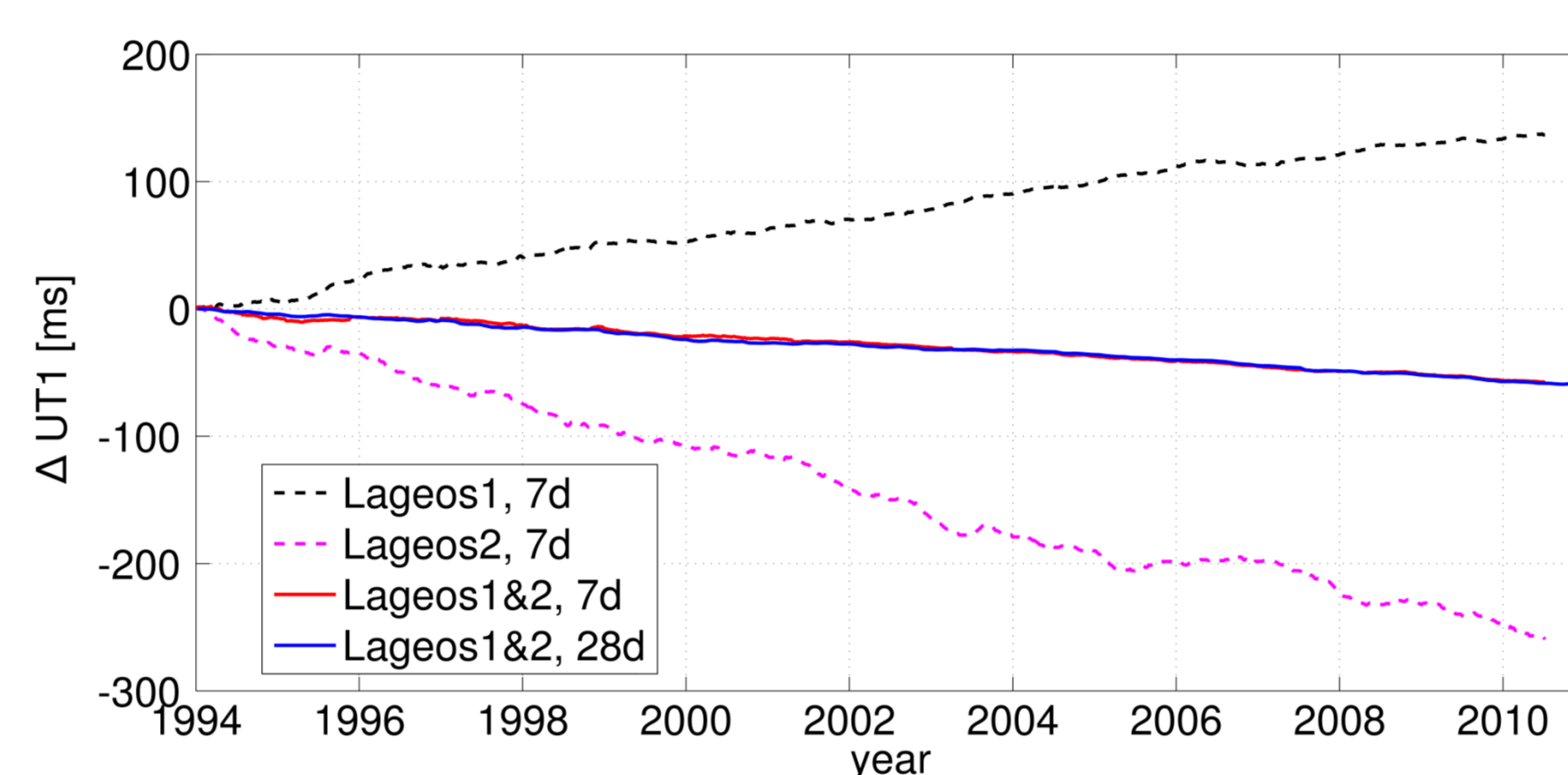
Fig. 3: Accumulated differences of UT1 w.r.t. IERS 08 C04 over a time span of 16.5 years. The individual solutions of LAGEOS 1 and 2 with an arc length of 28 days are not displayed (see Tab. 2).
