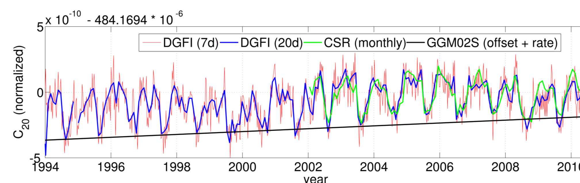
Fig. 4: Estimated normalized C_{20} coeffs. The DGFI solutions contain only data from LAGEOS 1 and 2 whereas the solution of CSR includes in addition data from Stella, Starlette and Ajisai.
