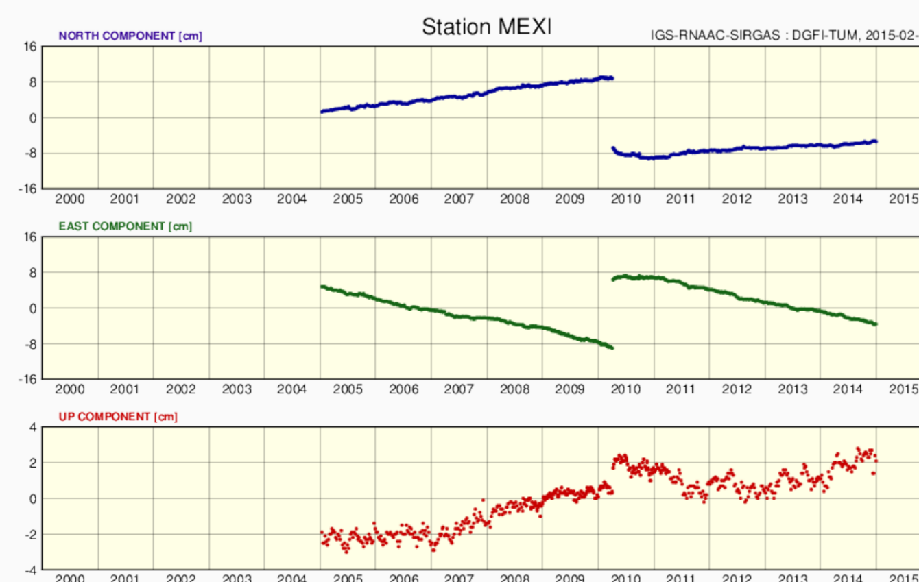
Fig. 3. Station position series at the SIRGAS station in Mexicali, Mexico.
