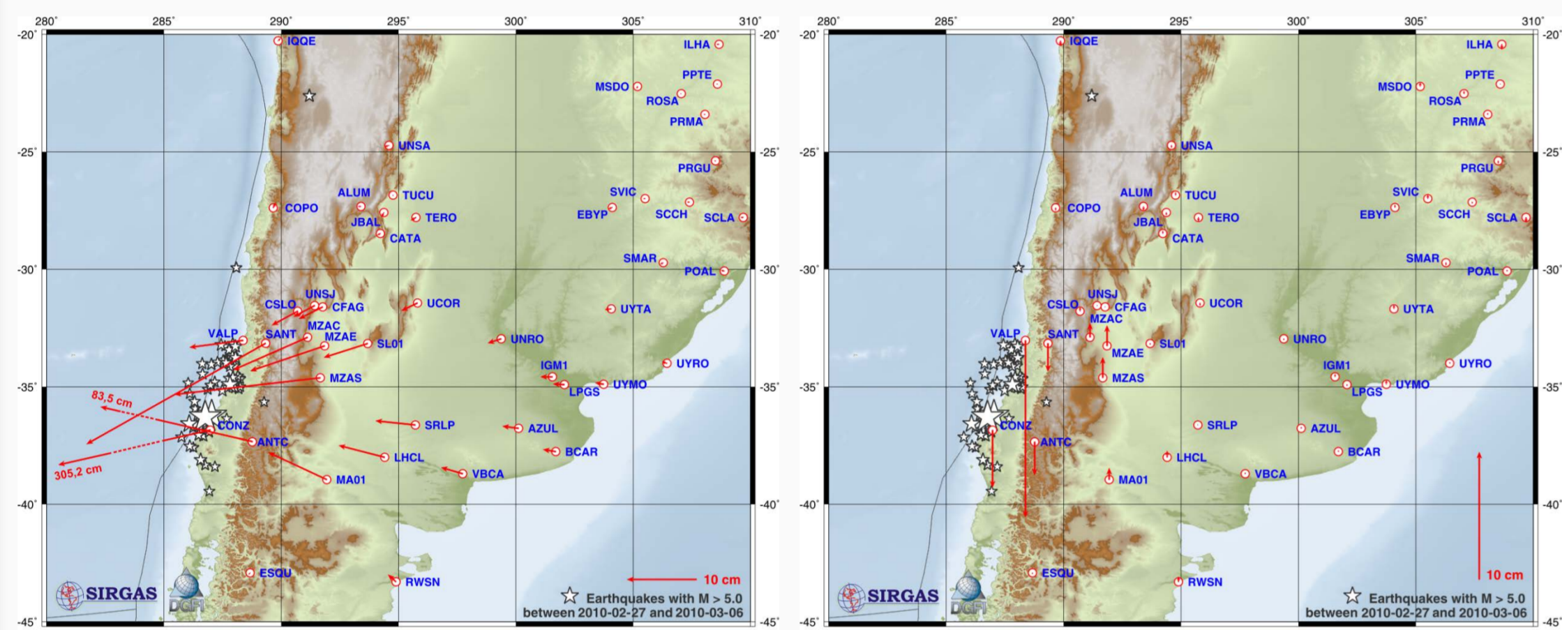
Fig. 1. Station displacements caused by the Maule earthquake on 2010-02-27.
