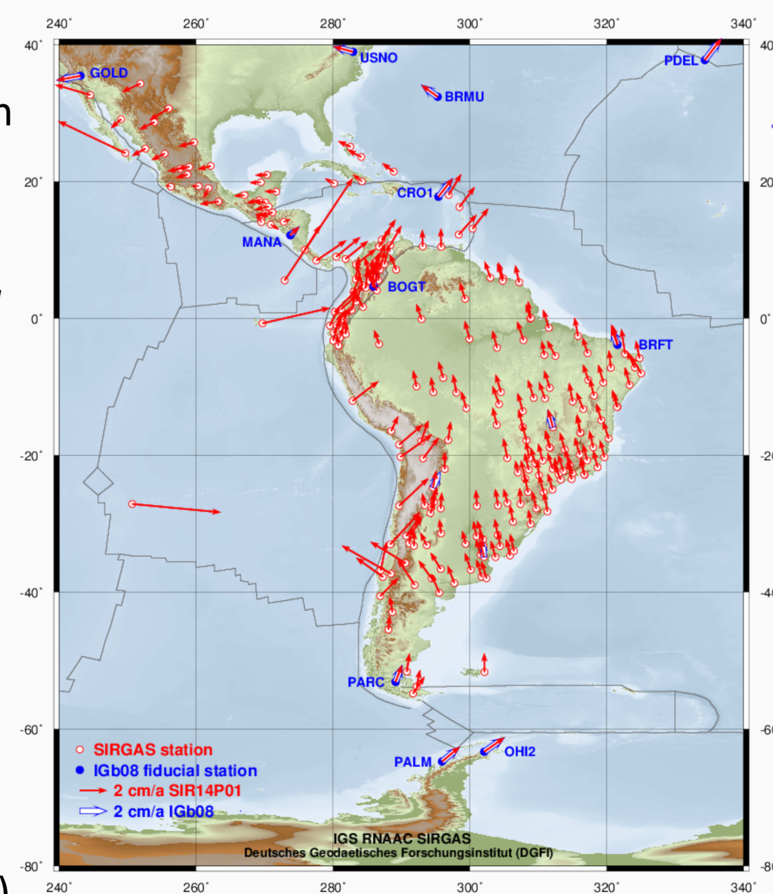
Fig. 5. Horizontal velocities of the post-seismic SIRGAS solution 2010-2014
