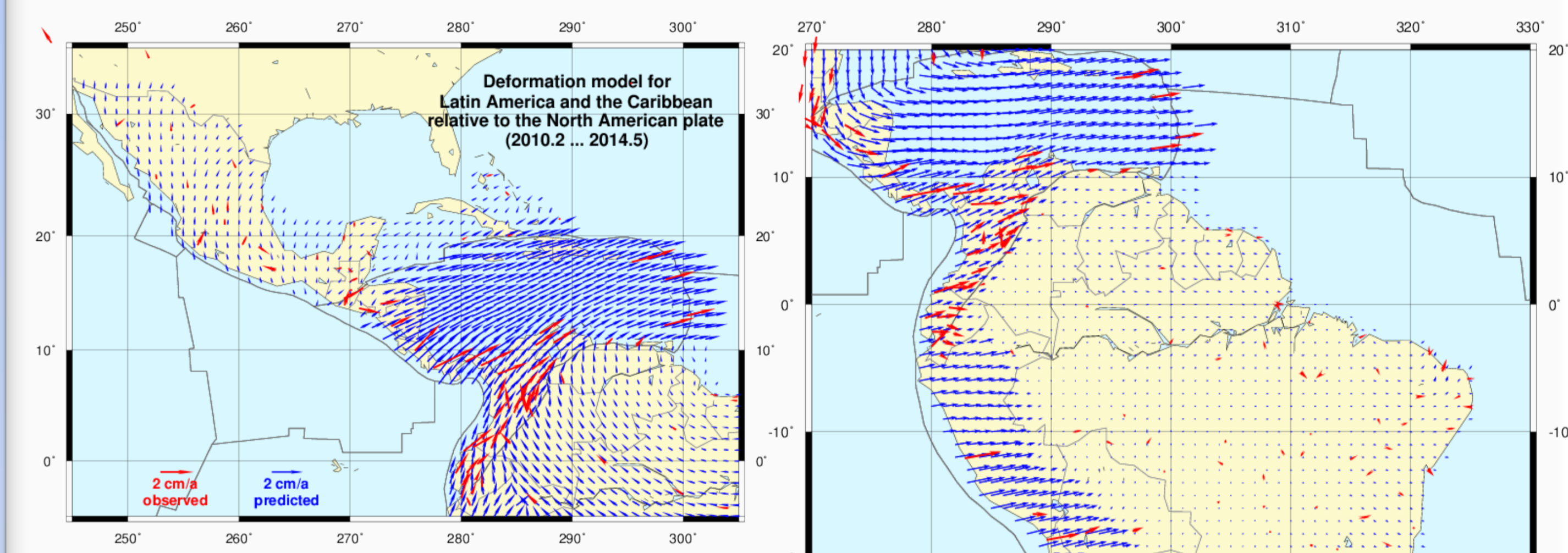
Fig. 6. Continuous deformation model (velocity model) for Latin America and the Caribbean 2010-2014 (VEMOS2014) relative to the North American plate.
