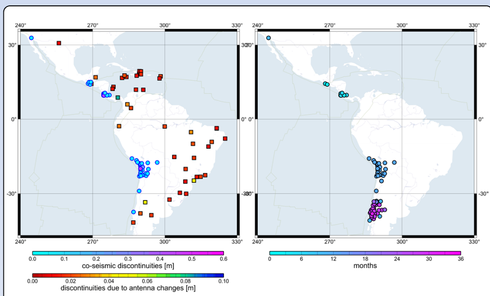
Fig. 5 – Station discontinuities (left) and post-seismic relaxation movements (right) identified in the SIRGAS reference stations from March 2010 to April 2015.
