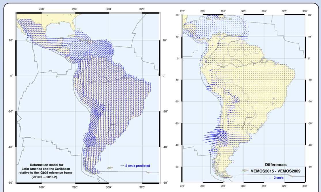
Fig. 6 – Post-seismic deformation model VEMOS2015 and its comparison with the pre-seismic model VEMOS2009.
