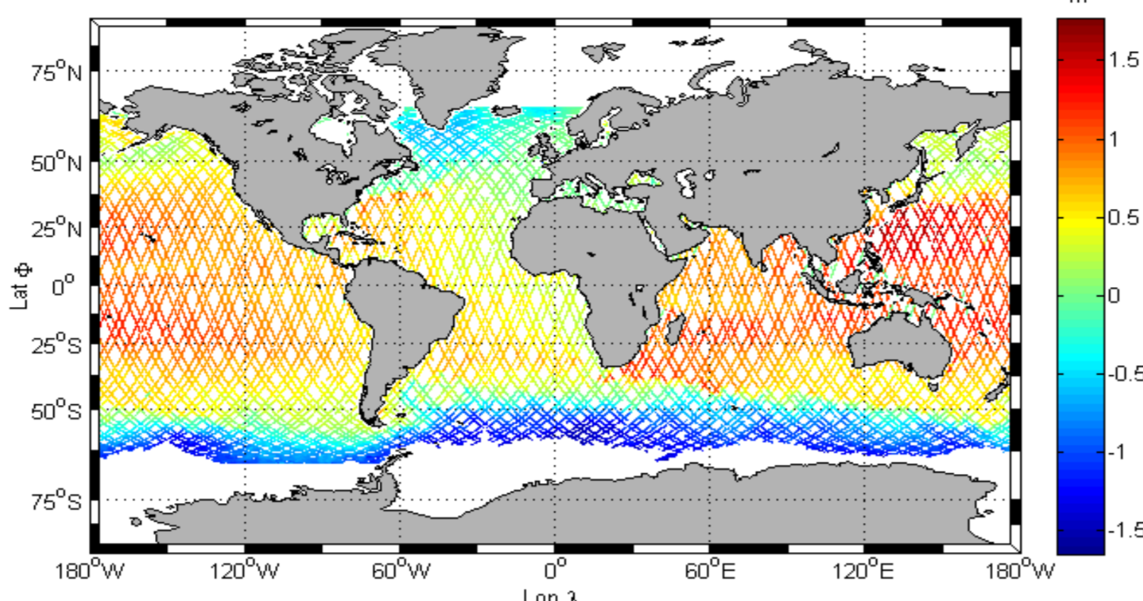
Fig. 1: The global iDOT profiles on the ground tracks of Cycle 36 from Jason-2 in June 2009.
