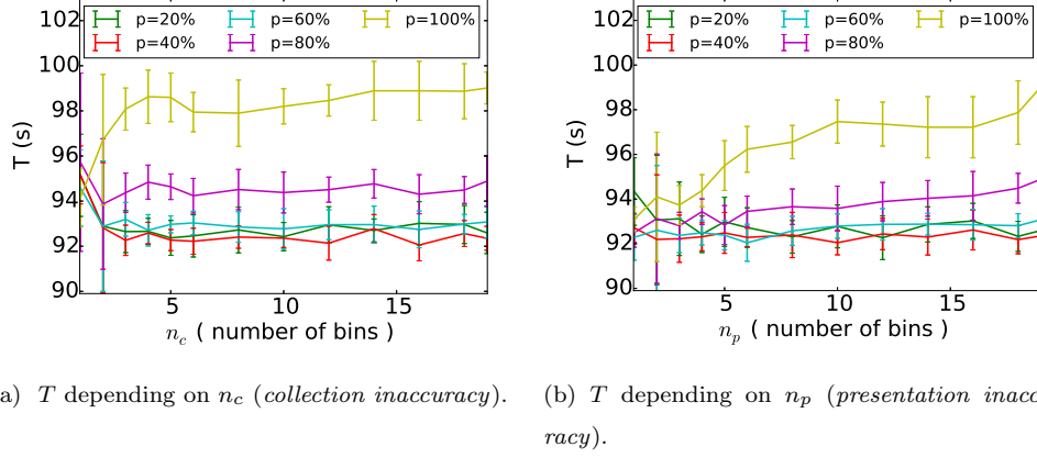
Figure 7: The average travel T (performance defined in Equation 1) depending on the inaccuracy or noise introduced either at collection or display, L_B = 875(m) , s = 100\% .
