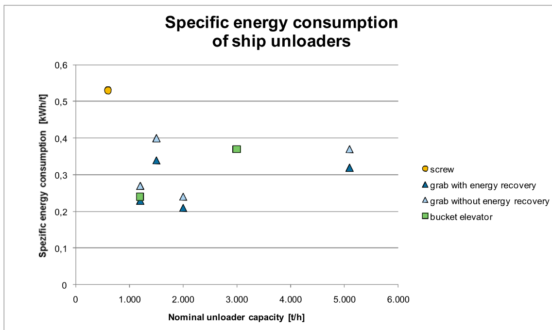
Fig. 15: Comparison of the specific energy consumption of all measured ship unloaders.
