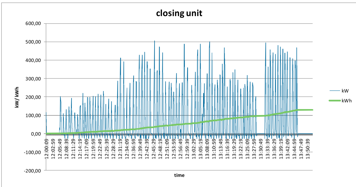
Fig. 12: Power/ power consumption diagram of the closure unit drive.
