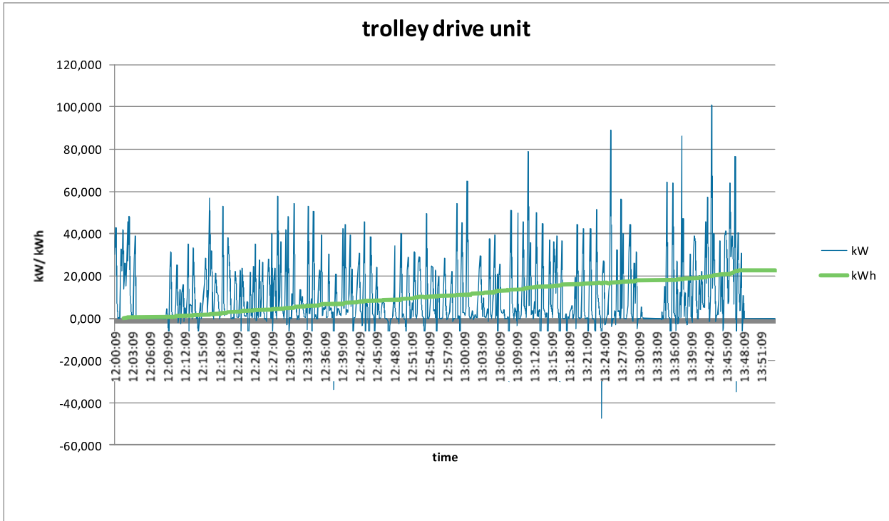
Fig. 13: Power/ power consumption diagram of the trolley drive unit.
