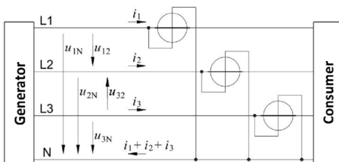
Fig. 7: Three wattmeter method to determine the power consumption in three-phase AC circuits. [4]
