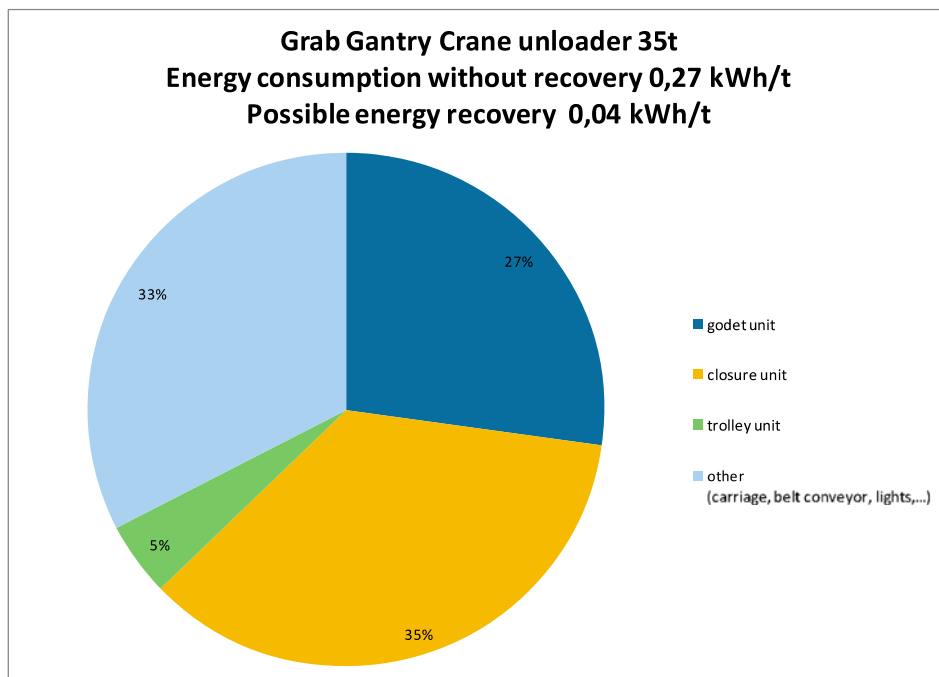
Fig. 14: Breakdown of the power consumption of the grab gantry crane unloader.
