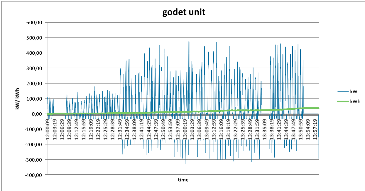
Fig. 11: Power/ power consumption diagram of the godet unit drive.
