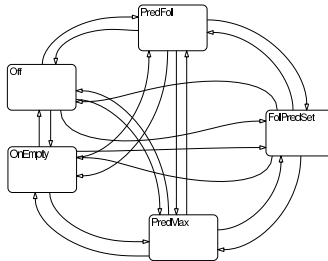
Figure 6: State machine of the discrete model
