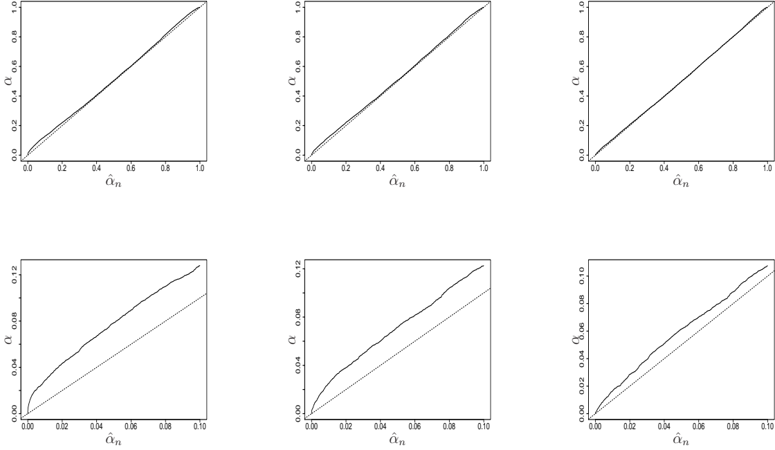
Figure 2: P-P plots for \sqrt{n}[\tilde{R}_n - \tilde{d}_n(\boldsymbol{\beta}_2, \boldsymbol{\beta}_3)] based on 10000 replications when \boldsymbol{\beta}_1 = (2, 2, 0.1, 0.1, 0.1)' , \boldsymbol{\beta}_2 = 2 , \boldsymbol{\beta}_3 = 2 errors are scaled t -distributed with 5 df (top row \alpha \in (0, 1) , bottom row \alpha \in (0, 0.1) ).
