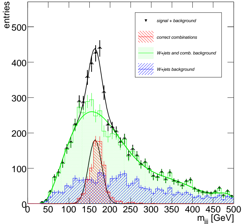
Figure 4.1: The invariant mass of the three chosen jets as a measure of the top quark mass. The blue histogram represents the W +jets samples, the red histogram shows the signal events with the correct three jet combination. The green histogram is the sum of W +jets background and the not correctly assigned signal events. The black points represent the total distribution. The results from the fitting procedure to the total simulated data are shown as curves: the Gaussian part in black, the Chebychev part in green, the upper black curve is the sum of both.
