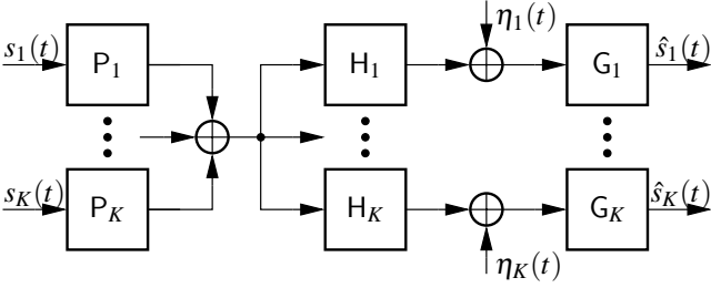
Figure 1: Broadcast Channel Model
