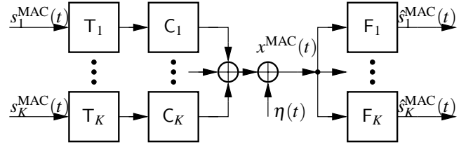
Figure 2: Multiple Access Channel Model
