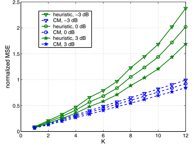
Fig. 2. MSE vs. K for different SNR (angular spread 10^\circ , f_d = 0.12 ).
