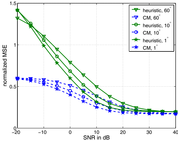
Fig. 1. MSE vs. SNR for different spatial correlations given by angular spread: \{1^\circ, 10^\circ, 60^\circ\} ( f_d = 0.12 , K = 6 ).
