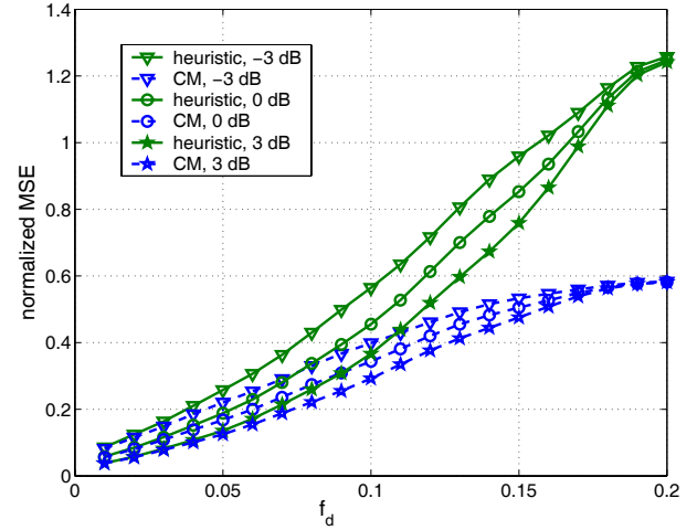
Fig. 3. MSE vs. max. Doppler frequency f_d for different SNR (angular spread 10^\circ , K = 6 ).
