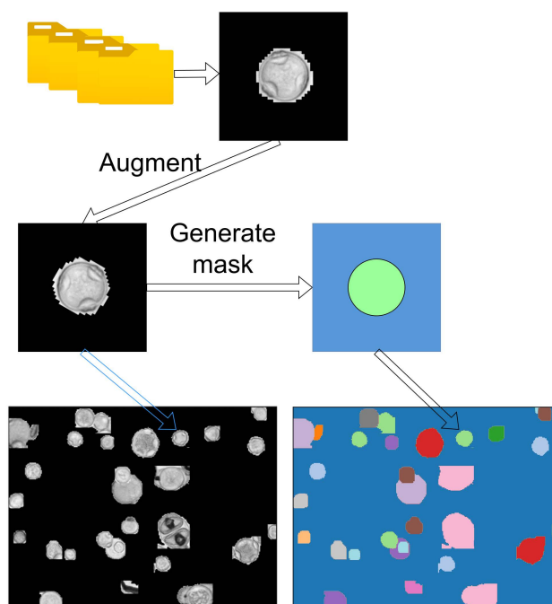
FIGURE 4. Cropped images are randomly selected from the data-set, augmented and used to create large synthetic images similar in complexity to the real images produced by the BAA-500.
