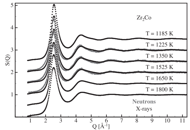
Fig. 2. Total structure factors S_N(Q) measured by neutron scattering (gray) and S_X(Q) measured by X-ray diffraction (black) for liquid Zr_2Co at different temperatures. The curves are shifted by multiples of 0.5 along the vertical axis.
