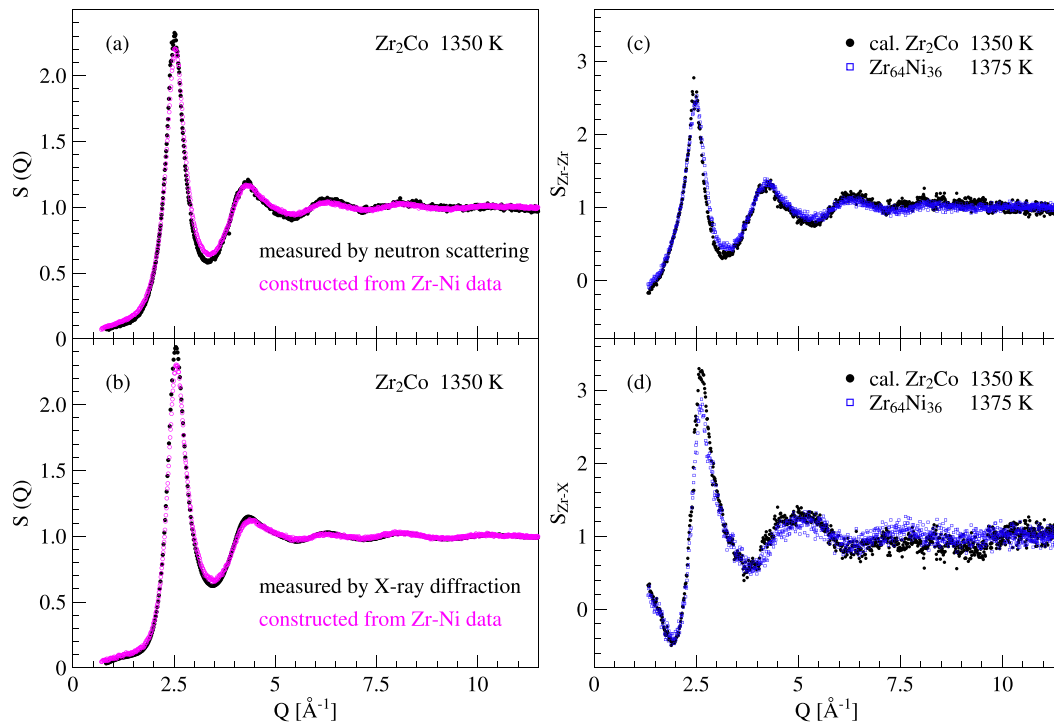
Fig. 3. Total structure factors measured by (a) neutron scattering and (b) X-ray diffraction for liquid \text{Zr}_2\text{Co} at T = 1350 K (black curves) and total structure factors constructed from the partial Faber-Ziman structure factors of \text{Zr}_{64}\text{Ni}_{36} melts assuming that the late transition metal component scatters like Co (pink curves). (c) and (d) show a comparison of the partial structure factors S_{\text{Zr-Zr}} and S_{\text{Zr-X}} ( X = \text{Ni}, \text{Co} ) in \text{Zr}_2\text{Co} and \text{Zr}_{64}\text{Ni}_{36} . For \text{Zr}_2\text{Co} these were calculated from the structure factors measured with neutrons and X-rays under the assumption that S_{\text{CoCo}} is the same as S_{\text{NiNi}} in \text{Zr}_{64}\text{Ni}_{36} . (For interpretation of the references to color in this figure legend, the reader is referred to the web version of this article.)
