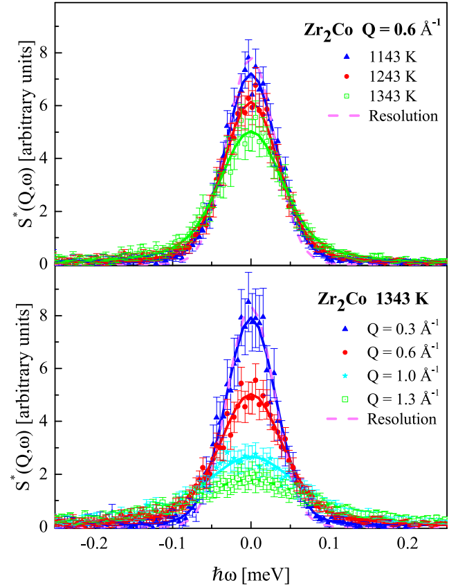
Fig. 6. (Color online) Quasielastic spectra for liquid \text{Zr}_2\text{Co} at Q = 0.6 \text{ \AA}^{-1} for different temperatures (upper part) and at T = 1343 K for four different wave vectors between Q = 0.3 \text{ \AA}^{-1} and Q = 1.3 \text{ \AA}^{-1} (lower part). The dashed line shows the instrumental resolution function measured on the vanadium standard. The solid lines show the fits with a Lorentzian function convoluted with the instrumental energy resolution.
