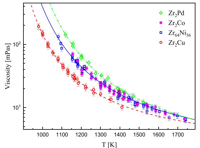
Fig. 9. Shear viscosity of liquid Zr_2Co (ref. [39]), Zr_{64}Ni_{36} (ref. [28]), Zr_2Cu , and Zr_2Pd (both this work) as function of the temperature.
