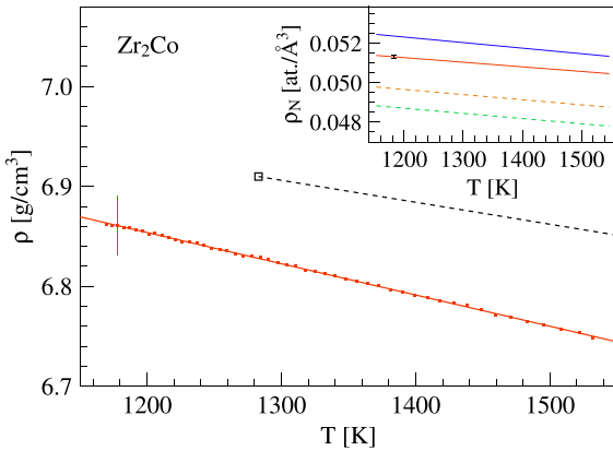
Fig. 5. Measured mass density of liquid \text{Zr}_2\text{Co} as a function of the temperature and a linear fit to the data points. The open square and the black dashed line show the density value and its temperature dependence obtained in the first-principles MD simulations of Huang et al. (ref. [31]). The inset shows the temperature dependence of the number density for liquid \text{Zr}_2\text{Co} (full red line), \text{Zr}_{64}\text{Ni}_{36} (full blue line, ref. [28]), \text{Zr}_2\text{Cu} (dashed orange line, ref. [16]) and \text{Zr}_2\text{Pd} (dashed green line, ref. [6]). Error bars show the uncertainty of the numeric values of the density, valid for all the measured data points. (For interpretation of the references to color in this figure legend, the reader is referred to the web version of this article.)
