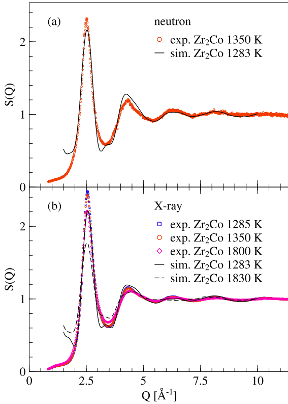
Fig. 4. Comparison between total structure factors for liquid \text{Zr}_2\text{Co} obtained by the first-principles molecular dynamics simulations of ref. [31] with those measured by neutron scattering (a) and by X-ray diffraction (b). The total structure factors of the simulation are calculated from the partial g(r) s using the corresponding neutron scattering lengths and X-ray scattering factors. For the neutron total structure factors the comparison is performed at a slightly different temperature as no experimental result is available at 1283 K. However, as it can be seen from the X-ray total structure factors, the temperature dependence is quite weak.
