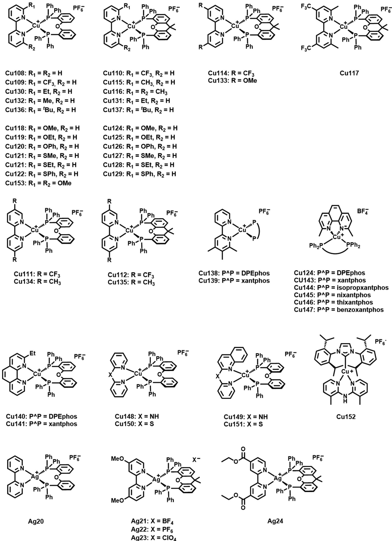
Scheme 7 Molecular structures of Cu108–152 and Ag20–24.
