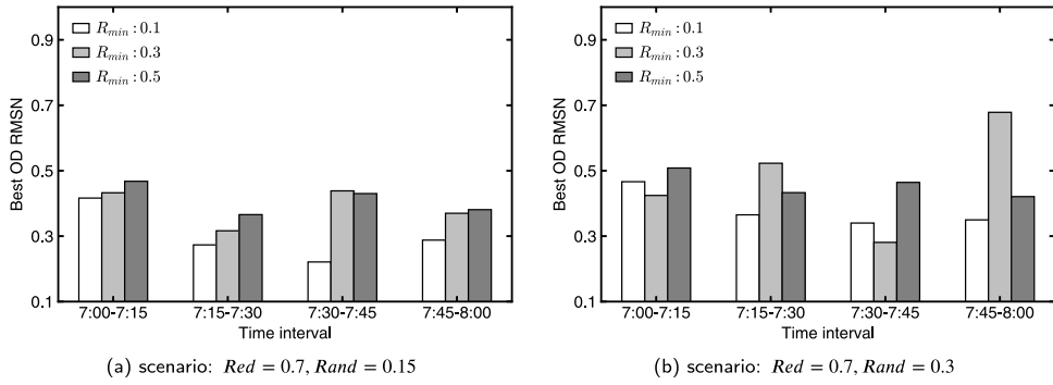
Fig. 19. OD RMSN with different R_{min} .
