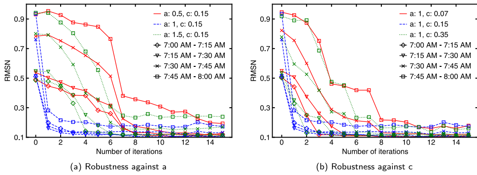
Fig. 13. Comparison of using different SPSA parameter values (c and a).
