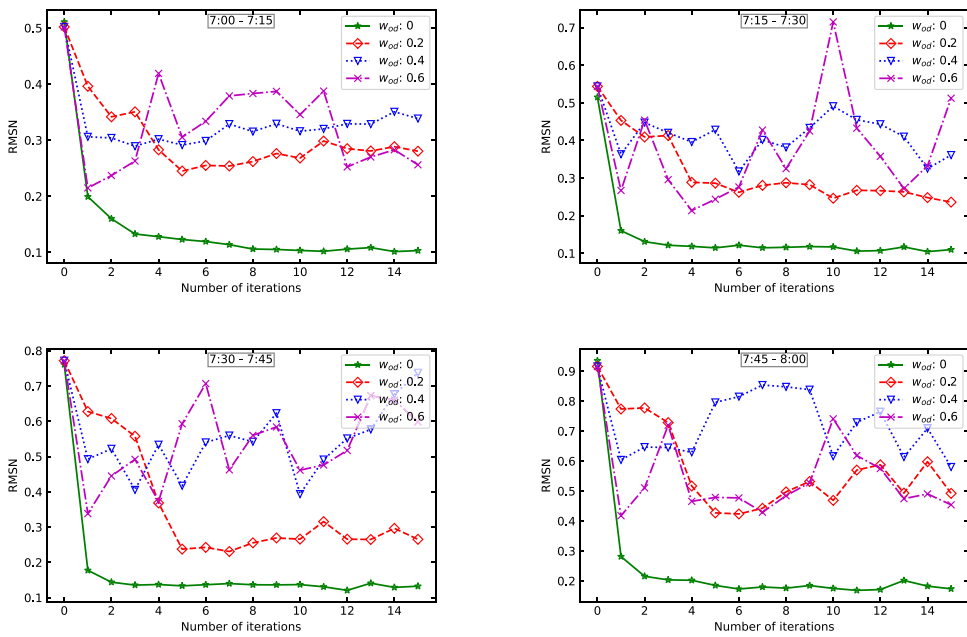
Fig. 11. Comparison between objective weights for specific intervals.
