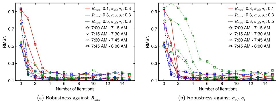
Fig. 17. Demand scenarios sensitivity (scenario: Red = 0.7, Rand = 0.15).
