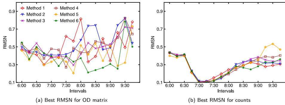
Fig. 9. Comparison between all generation methods.
