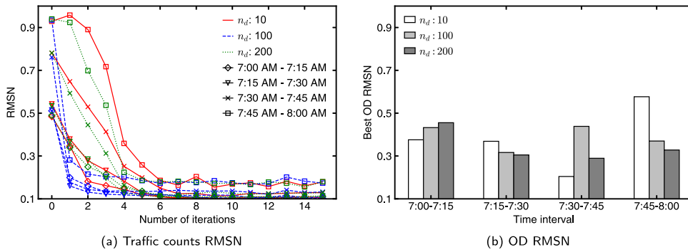
Fig. 16. Historical data matrices size sensitivity.
