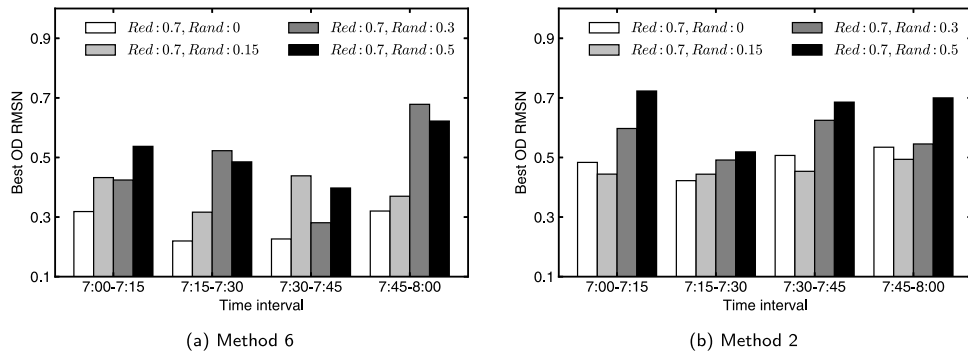
Fig. 15. Best OD RMSN of scenarios with different randomness.
