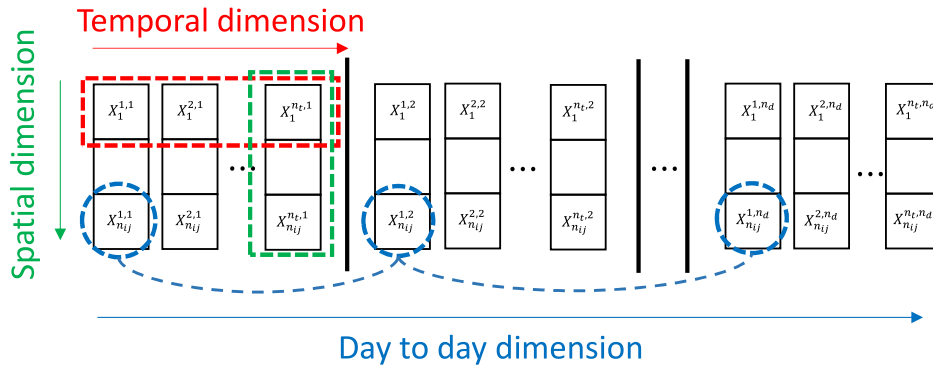
Fig. 1. Different correlation dimensions among time-dependent OD flows.
