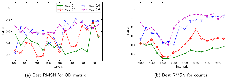
Fig. 12. Comparison between different weights combination in the objective function.
