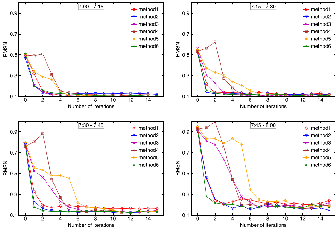
Fig. 5. Comparison between generation methods for specific intervals.
