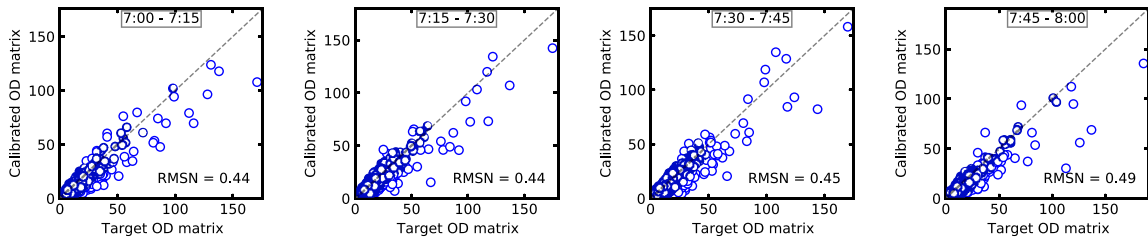
Fig. 10. Comparison of target and calibrated OD matrices (method 2).
