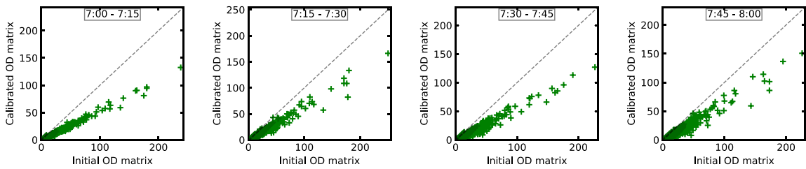
Fig. 8. Comparison of initial and calibrated OD matrices.
