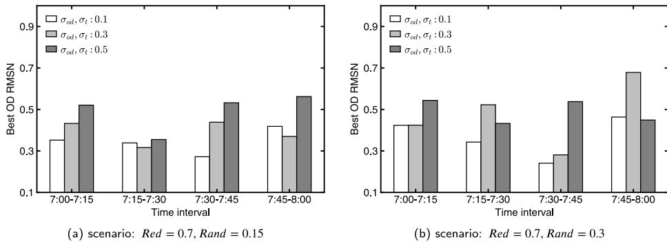
Fig. 20. OD RMSN with different \sigma_{od} and \sigma_t .
