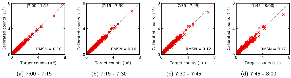
Fig. 6. Comparison of target and calibrated traffic counts.
