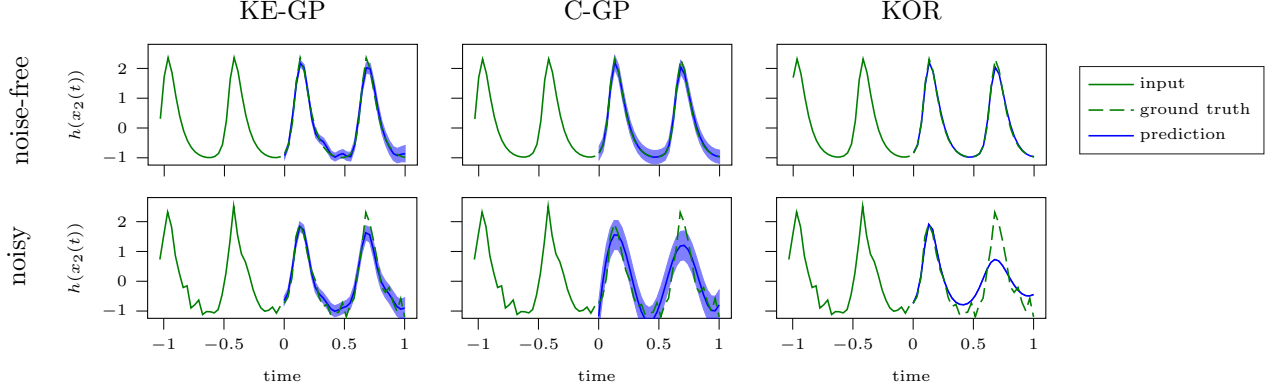
Figure 2: Multi-step mean and 2-sigma interval of the prediction for predator population from the predator-prey dynamics for our proposed Koopman-equivariant GP (KE-GP), a generic contextual kernel (C-GP), and a Koopman operator regression approach (KOR) for noise-free (top) and noisy (bottom) training data.
