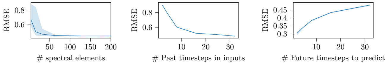
Figure 5: Ablation Studies: test RMSE with varying data and spectral parameters; we report mean and interquartile range over 10 runs.
