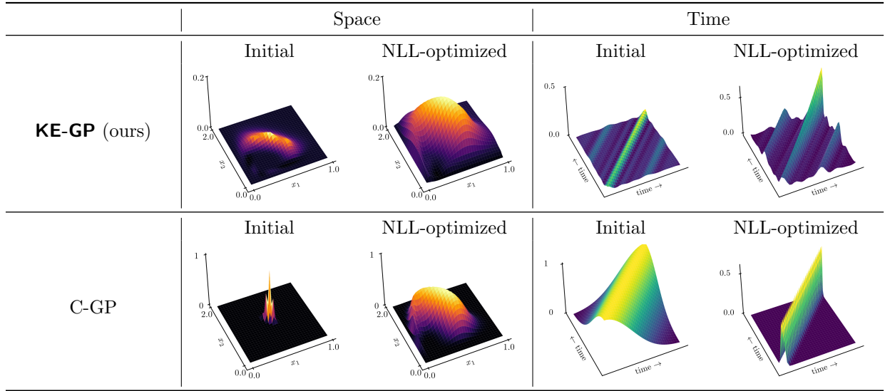
Figure 4: Visualization of the GP covariances in space and time. The spatial, KE-GP prior already strongly indicates the shape of the NLL-optimized covariance.
