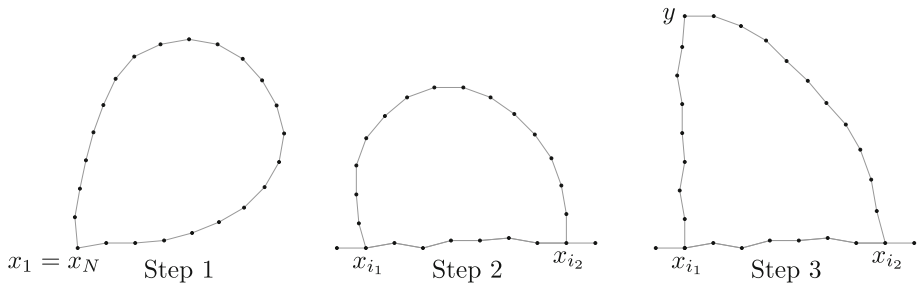
Fig. 5 The three cases discussed in Steps 1–3
