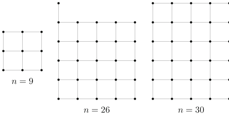
Fig. 2 Configurations of minimal energy for different cardinality
