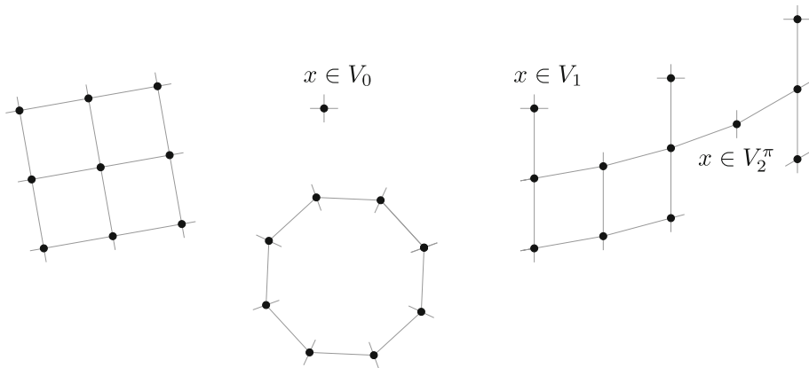
Fig. 3 Illustration of some strata in the bond graph of G . Degenerate strata are indicated by short segments crossing the atoms
