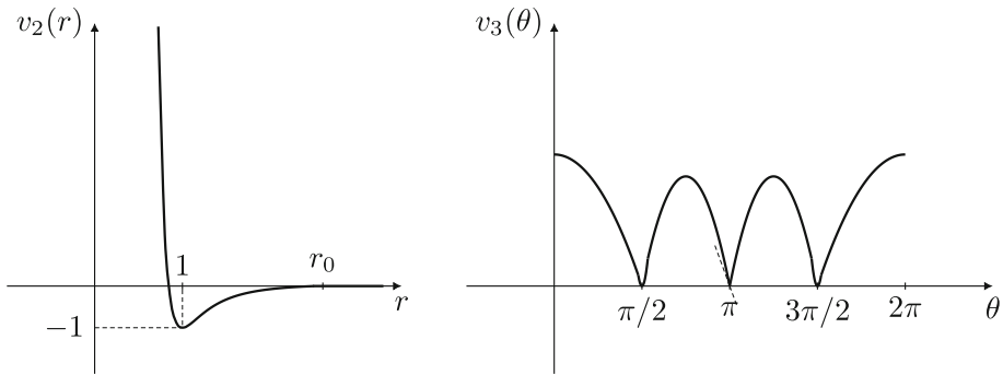
Fig. 1 The potentials v_2 and v_3
