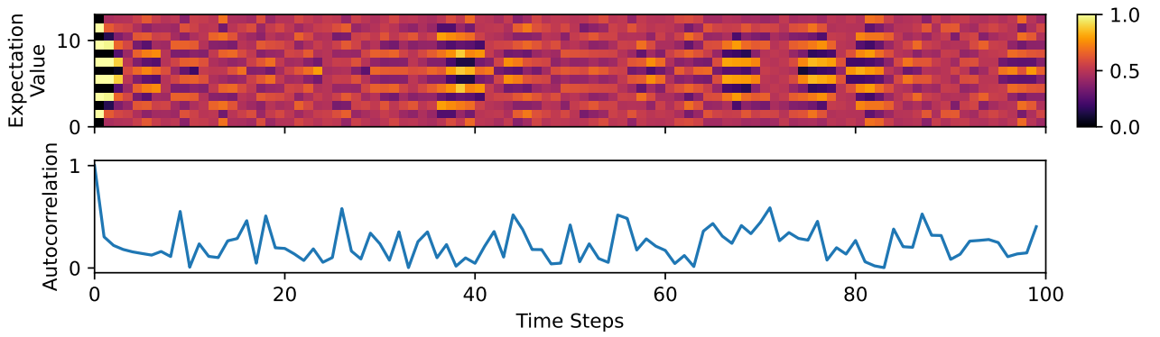
(c) Initial state: |0101010101010\rangle Boundary conditions: periodic
