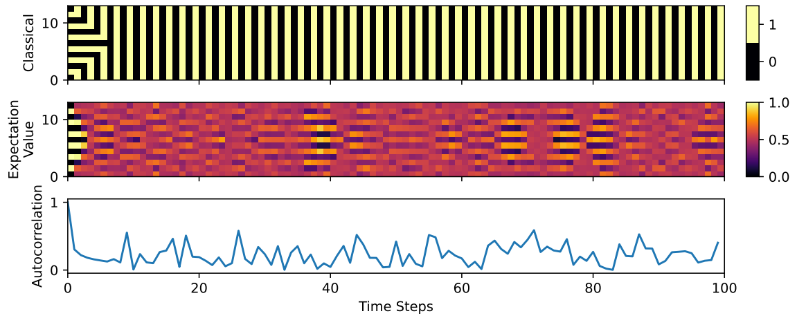
(c) Initial state: |0101010101010\rangle Boundary conditions: periodic
