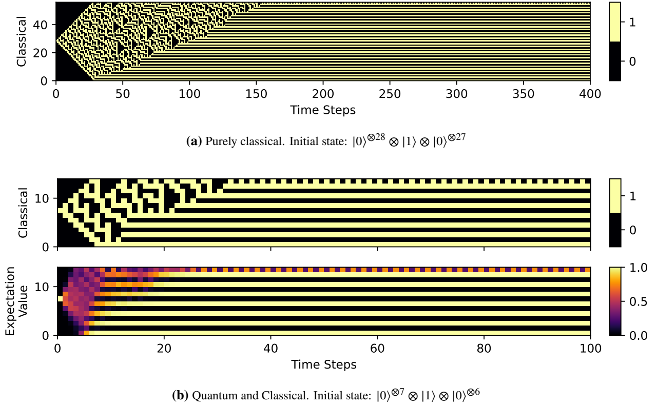
Figure 4.2 Comparison of the classical and quantum versions of the rule 30 elementary CA for different initial states
