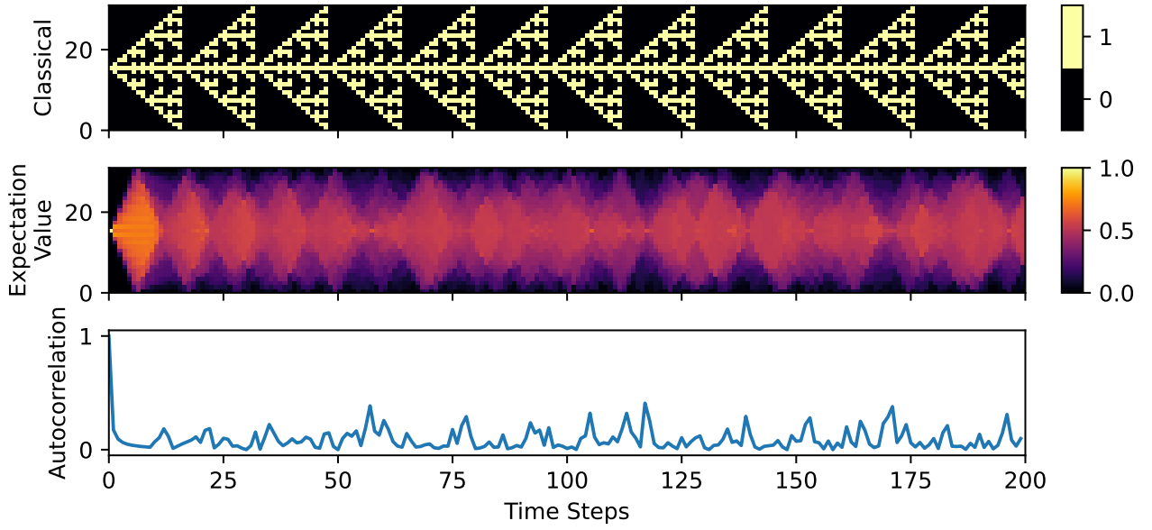
Figure 4.3 Comparison of the classical and quantum versions of the rule 150 elementary CA for the initial state |\psi\rangle_0 = |0\rangle^{\otimes 15} \otimes |1\rangle \otimes |0\rangle^{\otimes 15} . Autocorrelation is calculated as: |\langle\psi|_0|\psi\rangle_t| .
