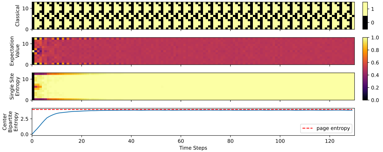
Figure 4.5 Time evolution of the rule 150 QCA with initial state |0\rangle^{\otimes 6} \otimes |1\rangle \otimes |0\rangle^{\otimes 6}
