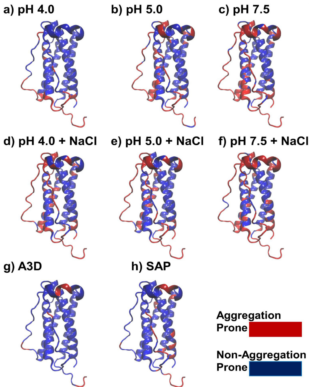
Fig. 9. The aggregation-prone residues determined from the CG simulations and prediction algorithms based on the PDB structure. a)-f) Interacting residues determined from the CG simulations. Aggregation-prone residues that were involved in the PPI in the CG simulations are colored red. Residues not prone to participate in aggregation (blue) interacted 25% or less compared to the strongest interaction at pH 4.0. g-h) Aggregation-prone residues are predicted from the initial PDB structure (PDB code: 1CD9) using aggrescan3d (A3D) and spatial aggregation propensity (SAP). Red residues represent aggregation-prone residues. Blue residues represent non-aggregation prone residues based on A3D-score or SAP lower than 25% of the strongest A3D/SAP score from 1CD9. (For interpretation of the references to color in this figure legend, the reader is referred to the web version of this article.)
