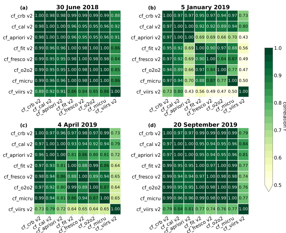
Figure 5. Tabular intercomparison of the correlations between the version 2 cloud fractions from ROCINN CRB, ROCINN CAL, OCRA a priori, the NO 2 fitting window (cf_fit), FRESCO, O 2 –O 2 , MICRU, and VIIRS for Europe and (a) the summer day, (b) the winter day, (c) the spring day, and (d) the autumn day.
