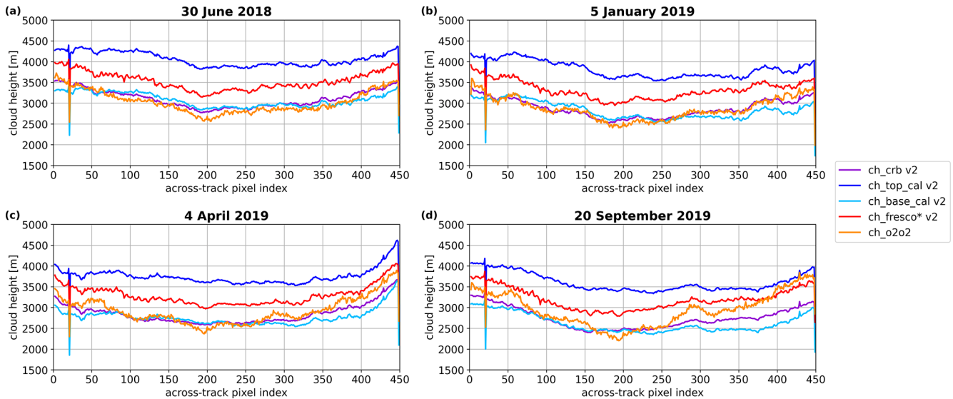
Figure 18. Mean values of version 2 cloud heights, as a function of the across-track index, from ROCINN CRB, ROCINN CAL top and base, FRESKO from the TROPOMI NO 2 product (ch_fresco*), and O 2 –O 2 for the globe and (a) the summer day, (b) the winter day, (c) the spring day, and (d) the autumn day with quality, snow, and ice flagging and only including pixels that have valid values for all products.
