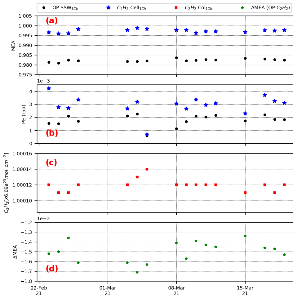
Figure 15. Time series of the MEAs, PEs, C_2H_2 retrieved column and difference between the MEAs retrieved with OP and cell method for the COCCON reference instrument SN37 ( a , b , c and d , respectively).
