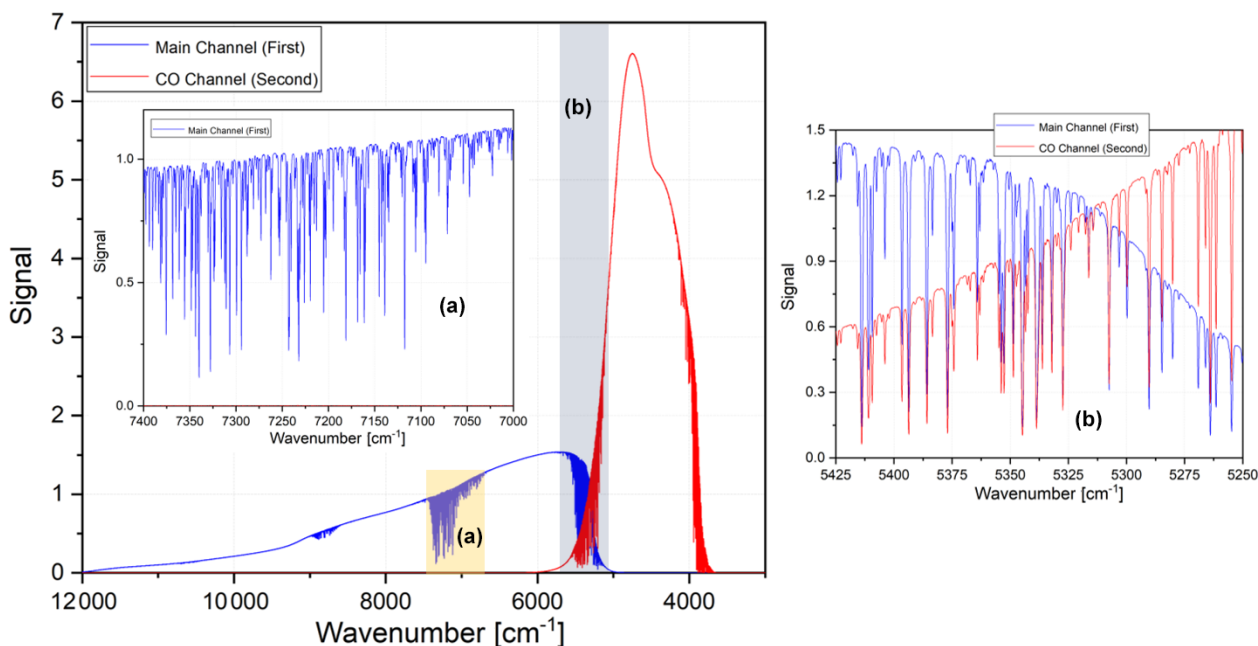
Figure 4. Typical spectra for both channels, obtained with the COCCON reference instrument SN37 on 19 March 2021. The highlighted regions (a) and (b) are the spectral windows used for the ILS retrievals.
