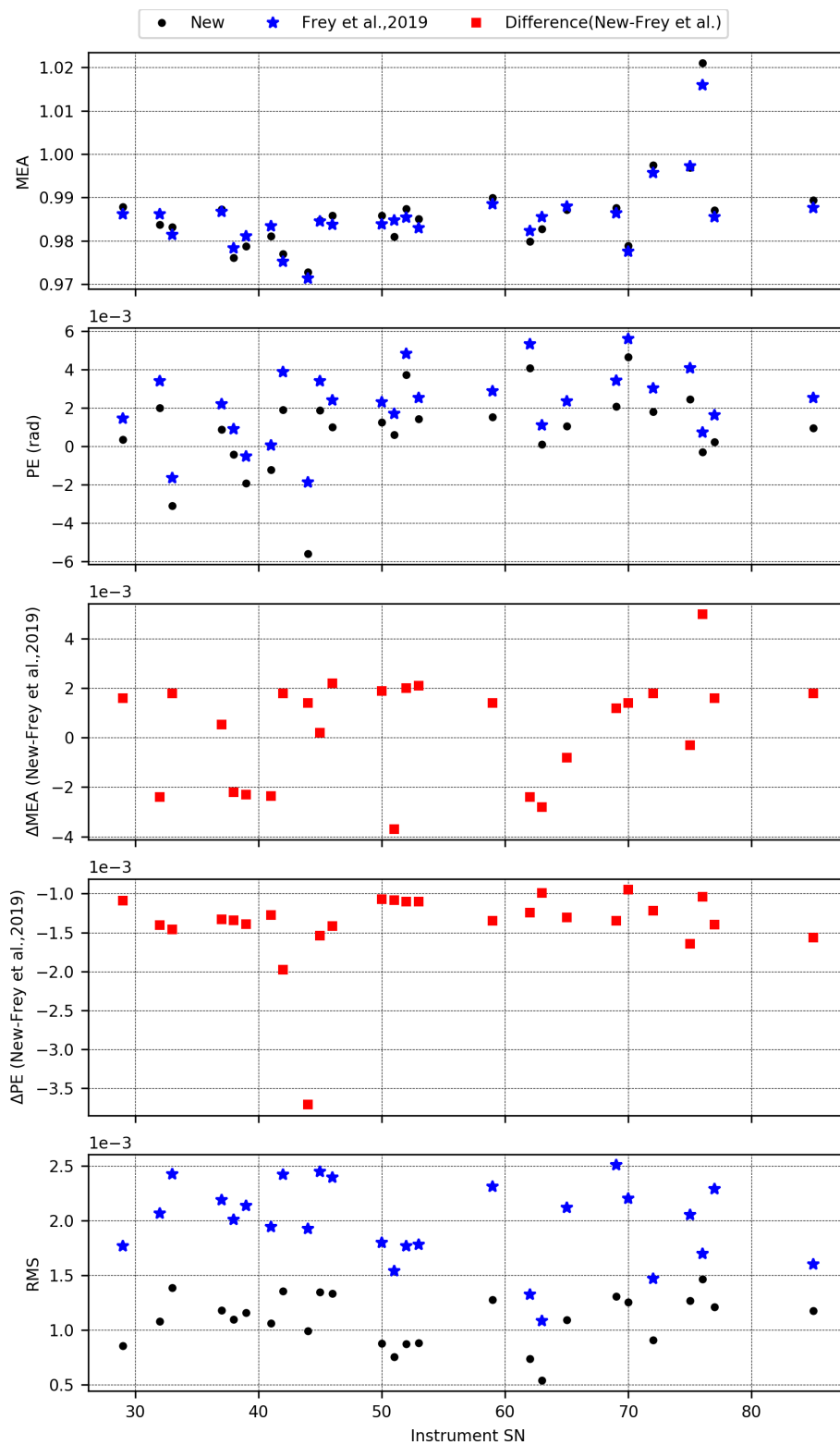
Figure 7. Comparison between the old published values (blue star) and the improved ones (black dots). The MEA, PE and new-minus-old difference for each spectrometer. The bottom panel shows the resulting empirical standard deviation of the spectral fit for the old and the new methods, respectively.
