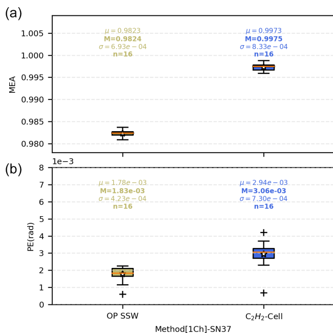
Figure 16. Same as Fig. 9 but for the sensitivity study for the COCCON reference instrument SN37. Left part of the display: open-path results; right part: cell results.
