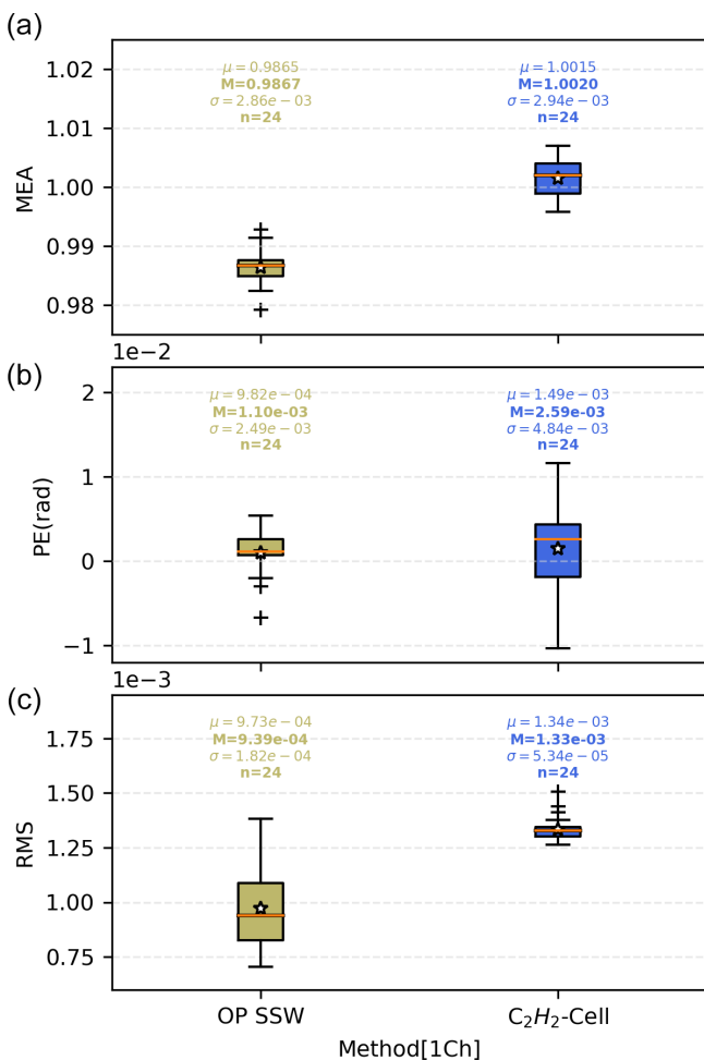
Figure 19. MEA and rms statistical results from the ILS retrievals by using the OP and the cell methods for the first channel of the available instruments (left part of the display: open path; right part: cell).
