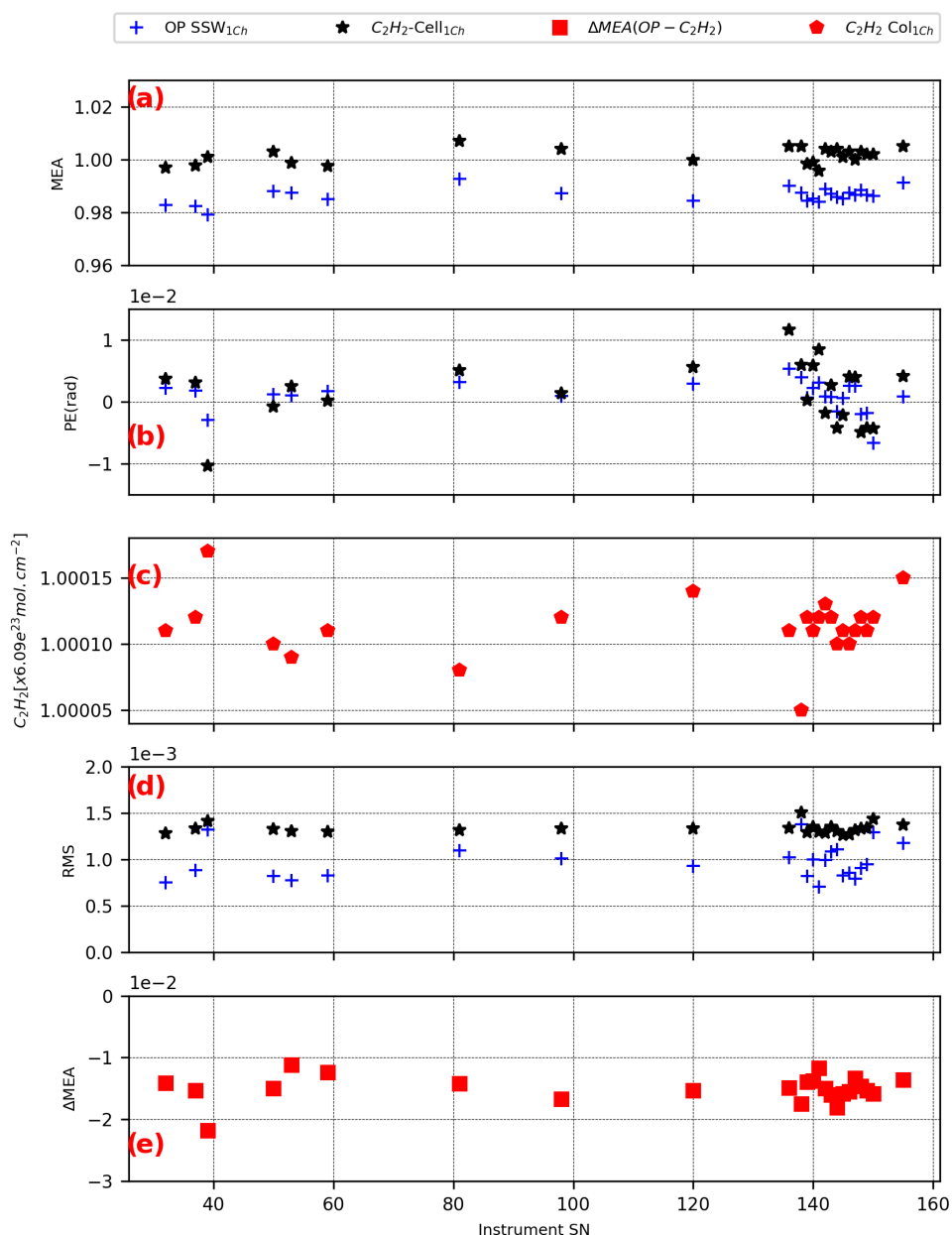
Figure 17. The modulation efficiency as a function of the instrumental SN, phase error, C_2H_2 column, rms of the spectral fit and the relative difference between the open-path method and the cell method are presented in (a), (b), (c), (d) and (e), respectively.
