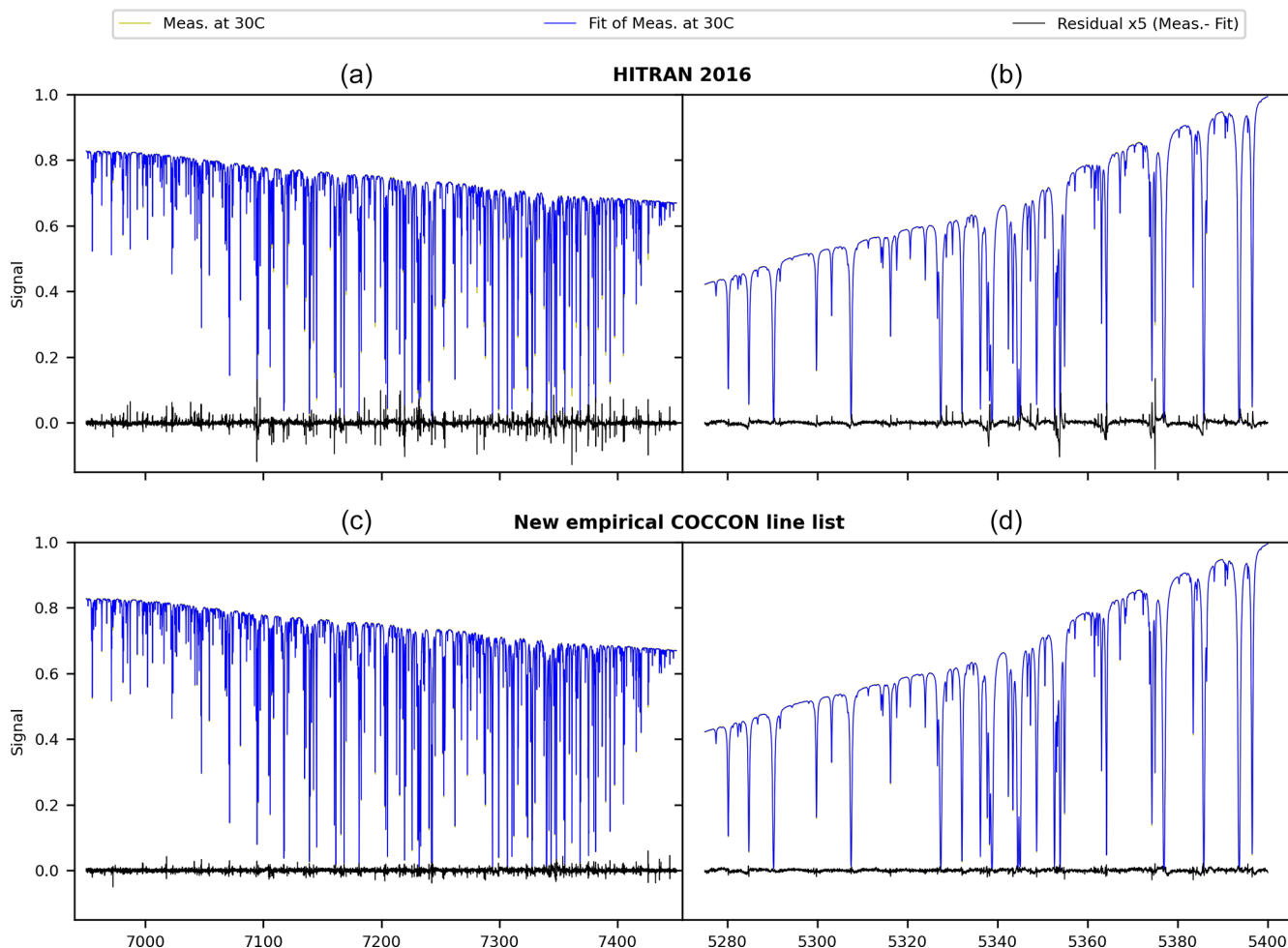
Figure A2. Same as Fig. A1, but the measured spectra were taken with the IFS125HR at KIT Karlsruhe, at 30 °C.
