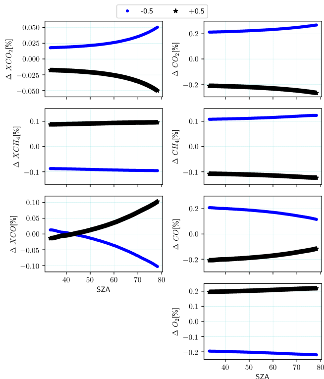
Figure 1. Variation in the relative difference for dry-air gas and total column gas amounts as a function of solar zenith angle (SZA), for changes in the original ILS of \pm 0.5\% of the original ILS parameters for COCCON's reference unit SN37 on 31 May 2021 at Karlsruhe, Germany, for carbon dioxide, methane and carbon monoxide, respectively, and the total column amount for oxygen.
