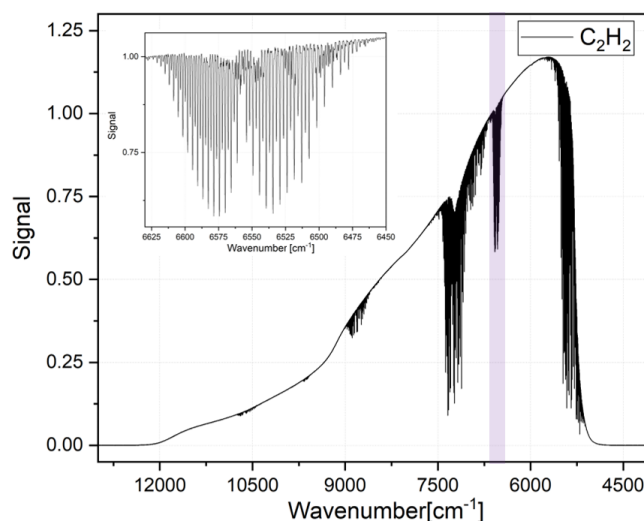
Figure 6. An open-path spectrum recorded with the \text{C}_2\text{H}_2 cell inserted in the beam. The spectrum was recorded using COC-COON's EM27/SUN reference spectrometer SN37. The insert shows a zoom-in of the wavenumber range used for the retrieval of ILS parameters from \text{C}_2\text{H}_2 .
