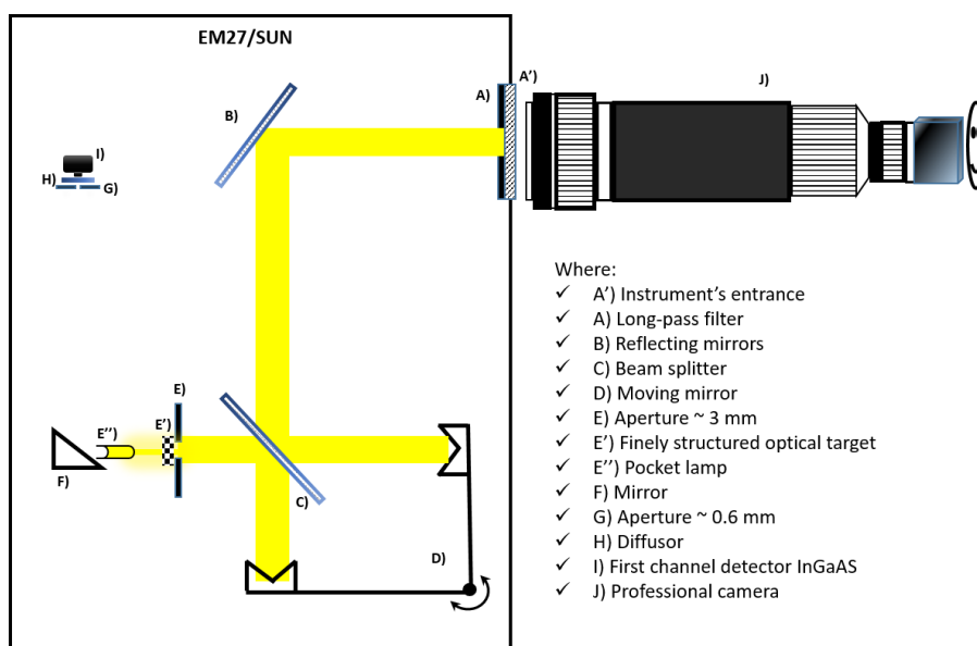
Figure 3. Light path of the beam inside the instrument coming from the lamp in E'' to the camera at the instrument's entrance A'.
