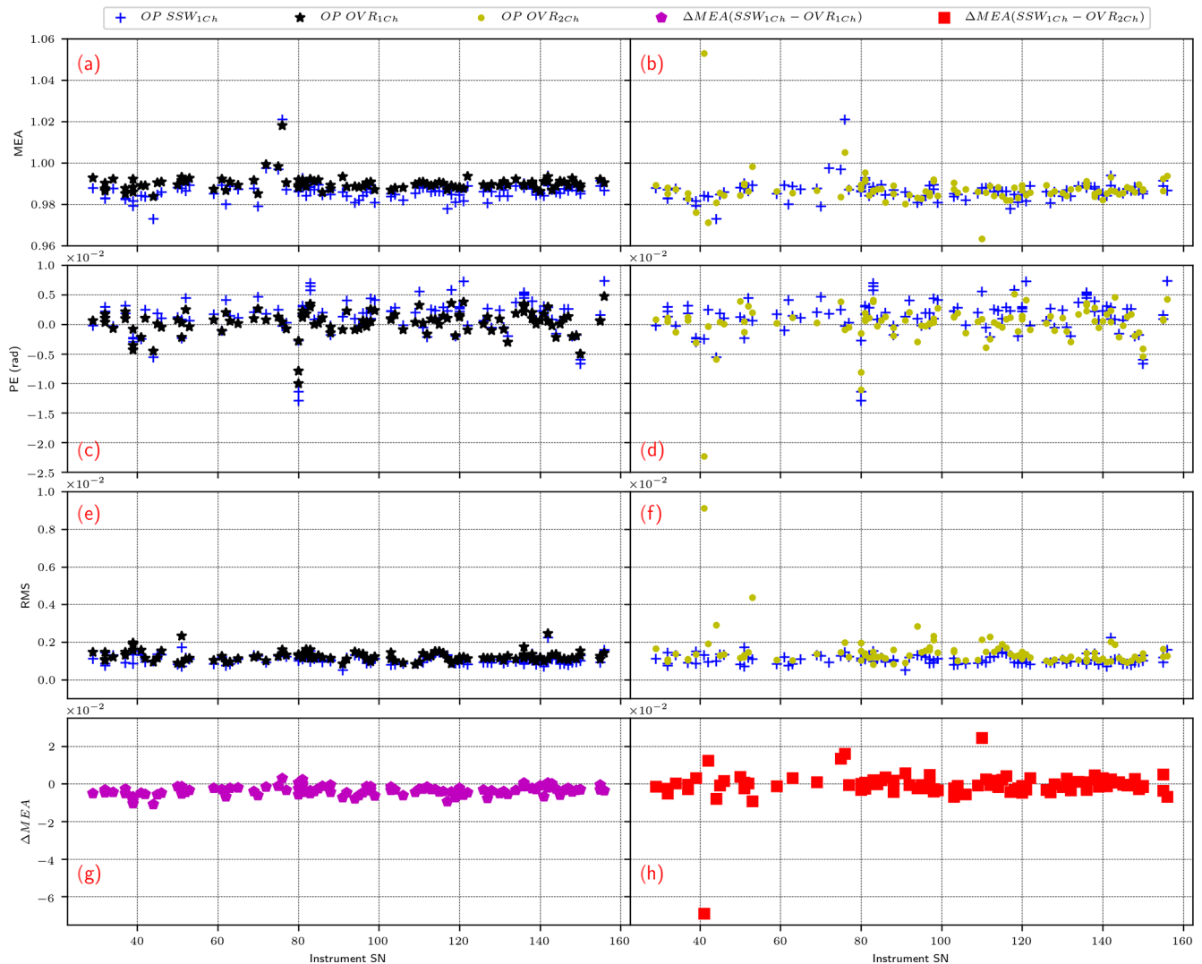
Figure 10. Main results for the main (a, c, e, g) and CO detector channels (b, d, f, h) resulting from the revised open-path method. The modulation efficiency, phase error, rms and relative difference for the first channel by using SSW and OVR are shown in (a), (c), (e) and (g), respectively, while the modulation efficiency, phase error, rms and relative difference for the first and second channels using SSW and OVR are presented in (b), (d), (f) and (h), respectively.
