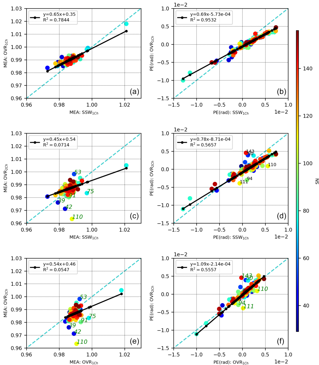
Figure 11. Correlation plots between the MEAs (a, c, e) and PEs (b, d, f). (a, b) The first channel in the SSW and in the OVR region, (c, d) the first channel in the SSW and the second channel in the OVR region, and (e, f) the first channel in the OVR and the second channel in the OVR region. Additionally, the obvious outliers are labelled in order to assess them.
