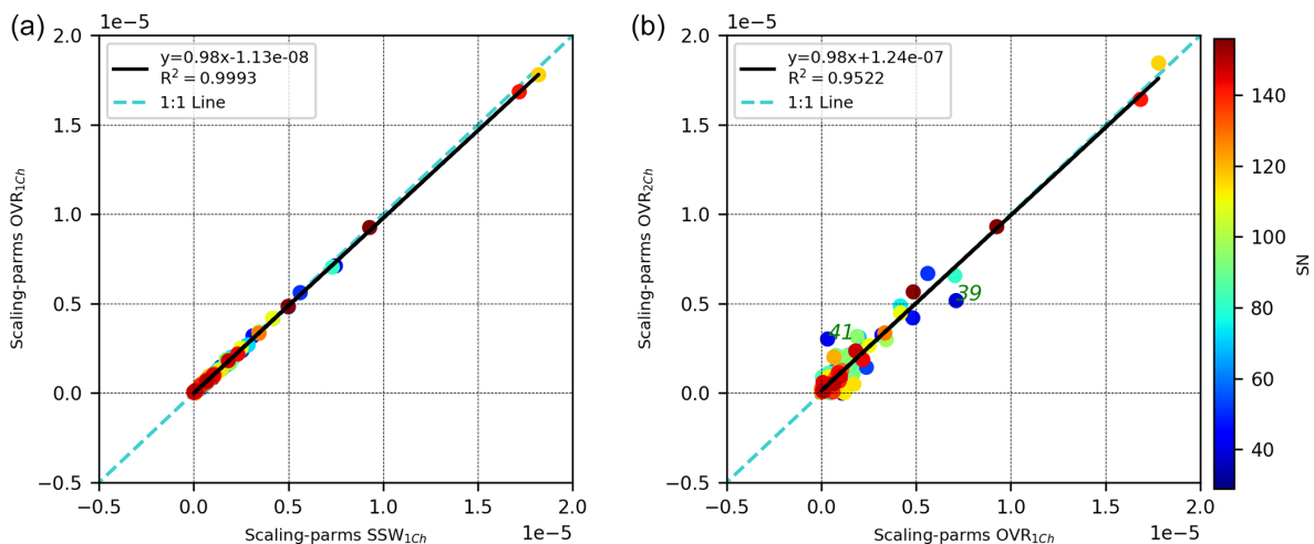
Figure 14. Correlations between the scaling factors derived from OVR and SSW spectral windows using the main channel spectra (a) and using CO channel results for the OVR spectral window (b).
