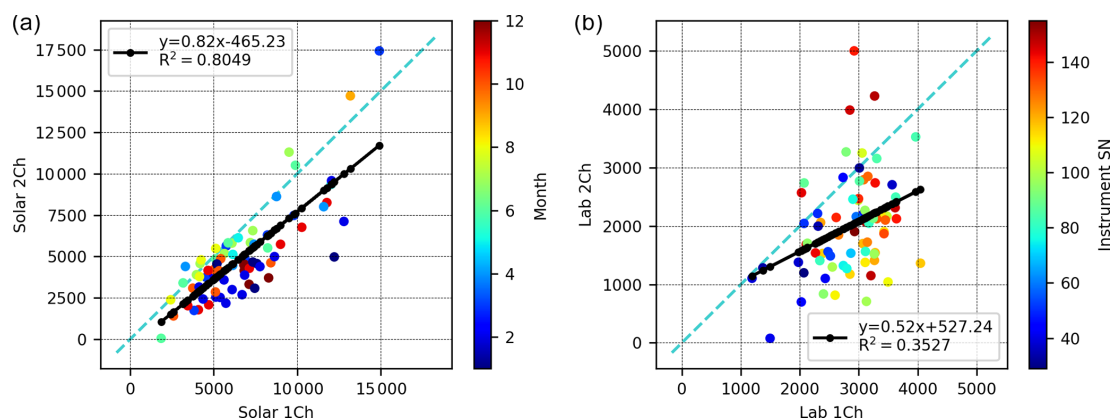
Figure 26. Correlations of the SNR obtained in channels 1 and 2, for the solar and OP measurements in (a) and (b), respectively. In (a) the colour code represents the month of the year when the solar measurements were carried out, for demonstrating the absence of an obvious seasonal signal in the SNR characteristics. In (b), the colour code represents the instrument's serial number because these measurements are carried out under controlled laboratory conditions by using a lamp as a light source. There might be a slight tendency towards higher SNR in recently built spectrometers.
