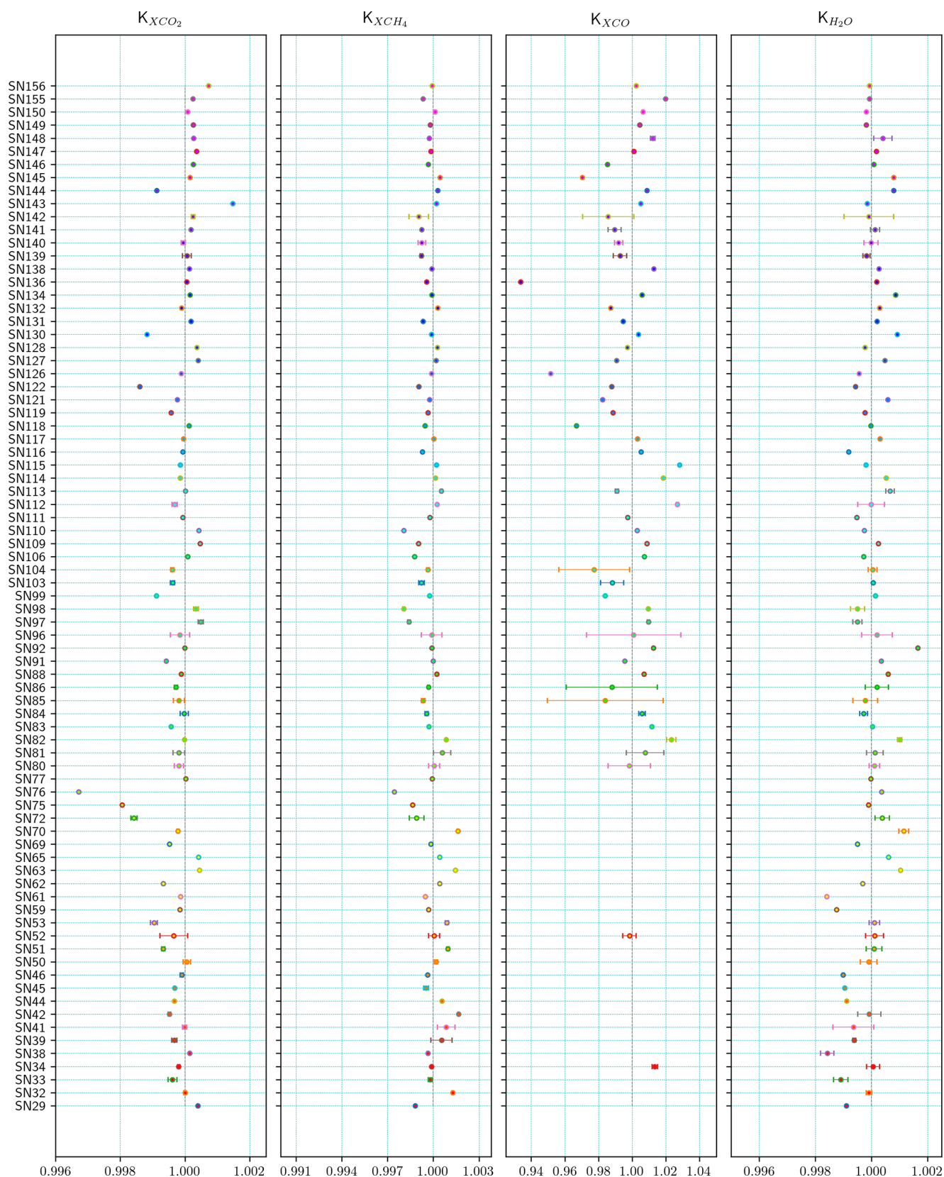
Figure 24. Correction factors for XCO_2 , XCH_4 , XCO and XH_2O from left to right, respectively, calculated for all EM27/SUN spectrometers. The error bar represents the standard deviation, and it is shown only for the instruments with more than one side-by-side measurement in Karlsruhe. The dashed line represents the ideal value “1.0” (practically realized by the COCCON reference spectrometer SN37).
