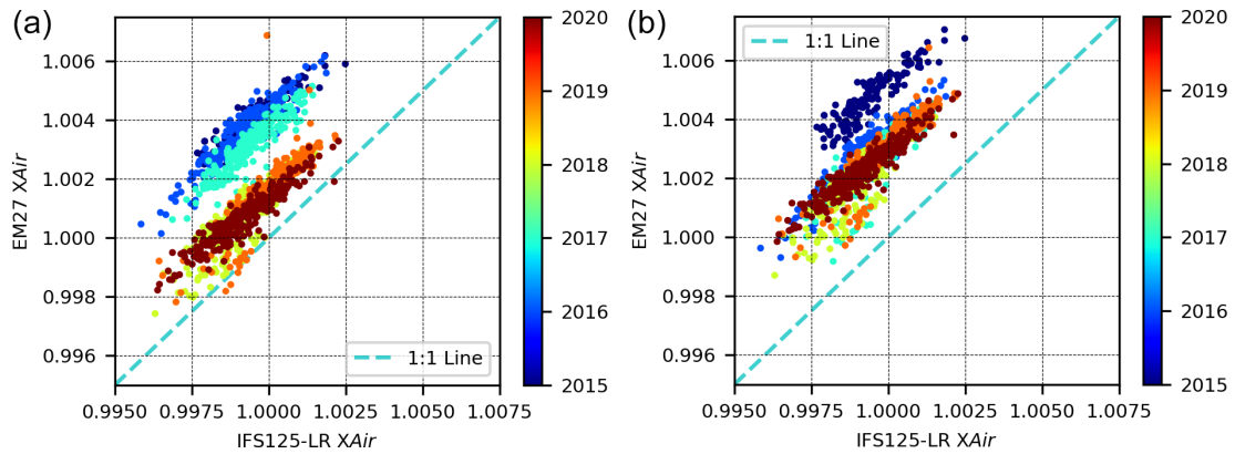
Figure 22. Correlations for the retrieved X_{AIR} by using the instrument SN37 and IFS125-LR. Panel (a) shows the results of the analysis of atmospheric spectra under the assumption of a constant ILS, and (b) shows the results under the assumption of a variable ILS (ILS parameters adjusted on a yearly basis).
