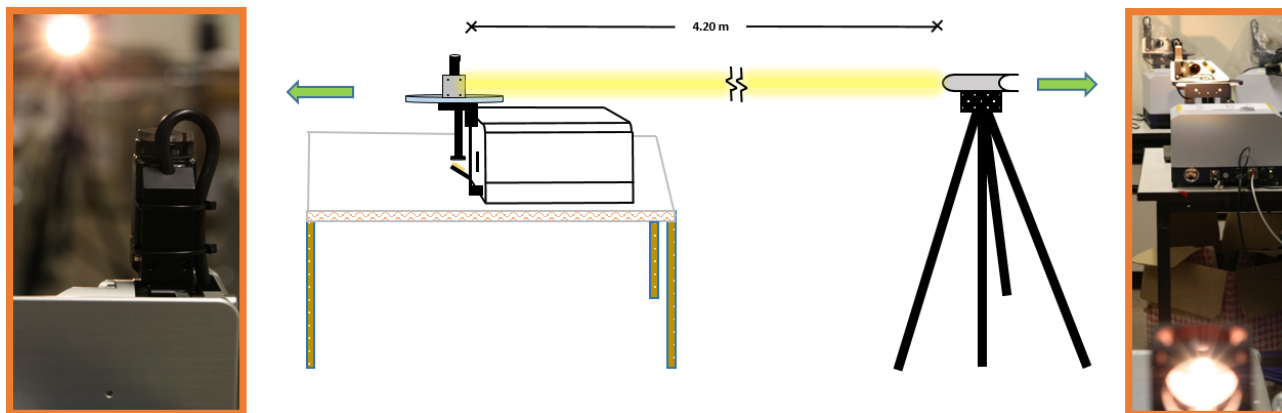
Figure 2. Set-up of the open-path measurements. The central part of the illustration schematically shows all the components and the alignment of the experimental set-up, while in left and right sides photographic close-up views are presented. The left photograph shows the view in the opposite direction from the spectrometer towards the lamp unit, while the right photograph shows a view from the lamp unit (bottom) towards the spectrometer with its solar tracker (top): the lamp in the bottom part and the instrument located at a distance of 4.20 m.
