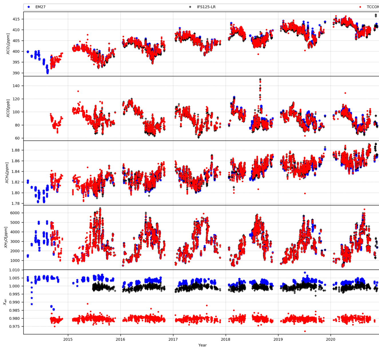
Figure 20. Time series of X_{\text{CO}_2} , X_{\text{CO}} , X_{\text{CH}_4} , X_{\text{H}_2\text{O}} and X_{\text{AIR}} measured with the COCCON reference instrument (blue), from the TCCON station Karlsruhe (derived from high-resolution IFS125-HR spectra using GGG2014, red) and derived from low-resolution IFS125-HR spectra (black). The low-resolution measurements were processed with PROFFAST.
