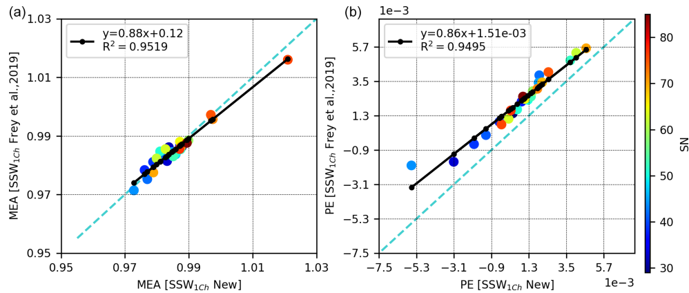
Figure 8. (a) Correlation between the MEA obtained with the new and the old methods for the shortwave standard micro window (SSW). (b) Correlation between the PE obtained with the new and the old methods. The colour bar represents the serial number (SN) of the instruments.
