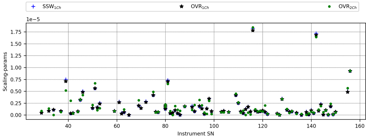
Figure 13. Instrumental variation in the spectral scaling factors in each of the spectral windows used and for both channels.
