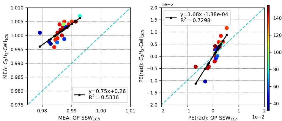
Figure 18. Correlations between the MEAs obtained with the OP and cell methods for the first channel.
