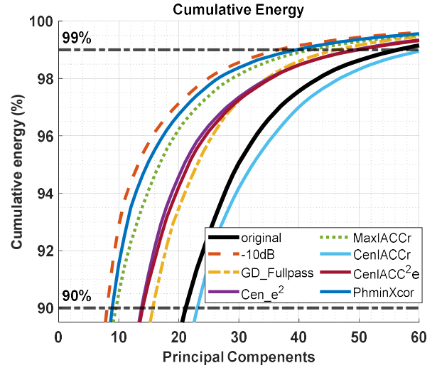
Figure 1: The plot represents the cumulative energy at specific numbers of principal components calculated from the PCA results of the original and preprocessed HRIRs using -10 dB relative threshold, group-delay, centroid of the squared envelope, maximum of the cross-correlation, centroid of the cross-correlation and its squared, and also cross-correlation of the minimum phase components of the signals. The cumulative energy is plotted for 60 principal components (out of 440) for ease of demonstration.
