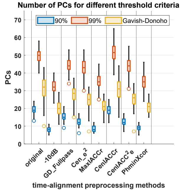
Figure 2: The distribution of the minimum number of PCs calculated for the three threshold criteria of 90 and 99 percent of cumulative energy and Gavish-Donoho across 92 subjects. Results are given for the seven delay calculation methods.
