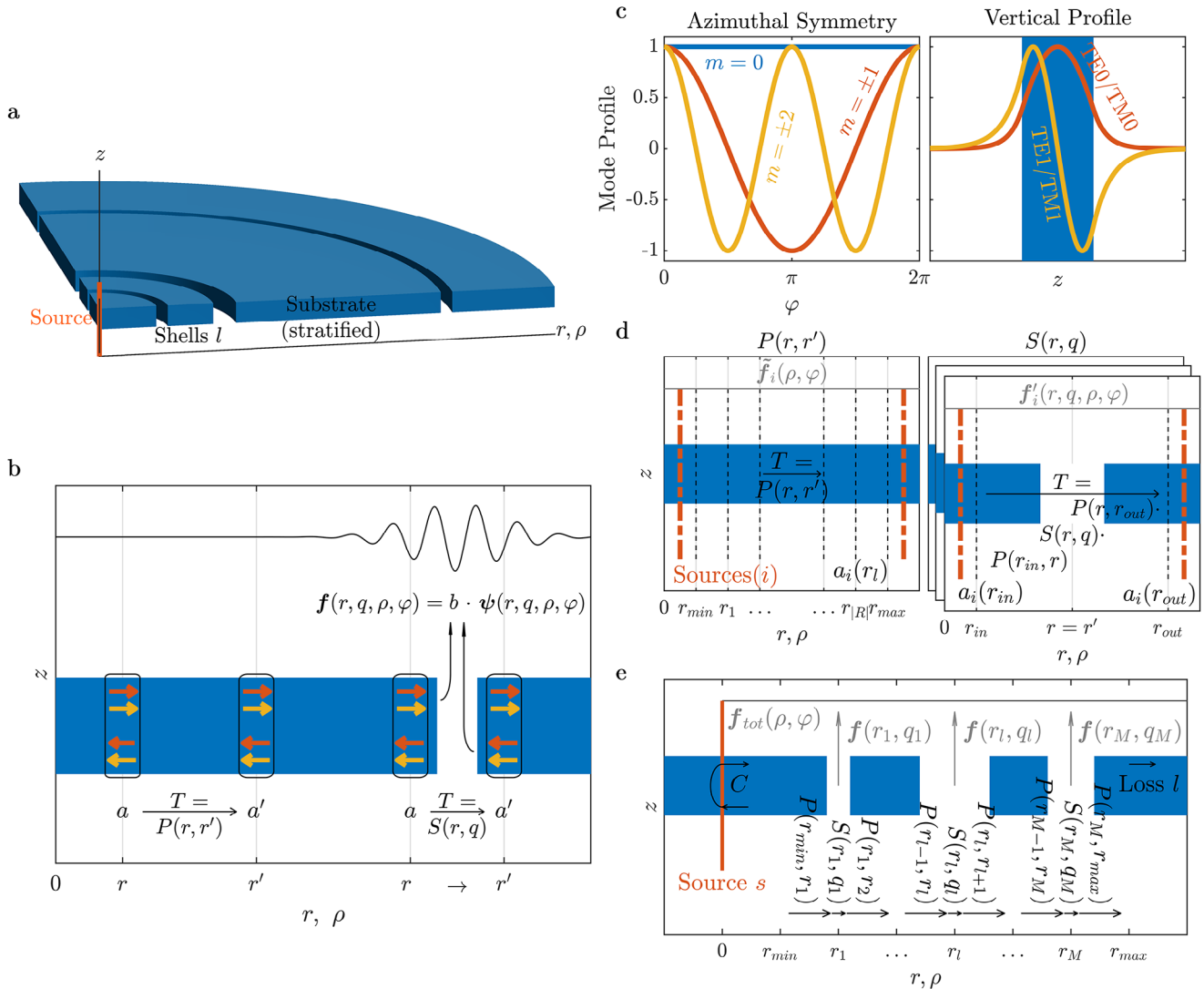
Figure 1. Concept of the the radial scatter transfer matrix model (rsTMM) a) Sketch of the structure to be simulated. A centered source is embedded into a (stratified) substrate, with concentric shells l of arbitrary scatterers surrounding it. b) Basic concept of the rsTMM. The substrate of interest supports modes (orange arrows), propagating inward or outward. The complex vectors a, a' give the mode amplitudes at a fixed radius r, r' . Propagation ( P , left), as well as scattering ( S , right) between the modes is described by transfer matrices T . Emission into free-space from modes impinging on a scatterer is described by fields f , which are calculated as linear combination scaled by the impinging mode amplitudes b (for details: see main text). c) The modes we consider are guided modes, characterized by the combination of their azimuthal symmetry (left) and their vertical profile (right) governed by the substrate. d) Transfer matrices are calculated from sets of simulations i , employing single mode sources at either the inner or outer position. The undisturbed substrate (left) yields all propagation transfer matrices P , a substrate with a single scatterer yields the scatterer transfer matrix S for this scatterer with geometry q at radius r (right). Simulations have to be repeated to form a database of different scatterers. e) The complete structure is assembled by multiplying the scatter S and propagation P transfer matrices, then applying boundary conditions for the source s , center reflection C and side-loss l . Finally, the coherent sum over the emission of all scatter shells gives the total free-space emission f_{tot} .
