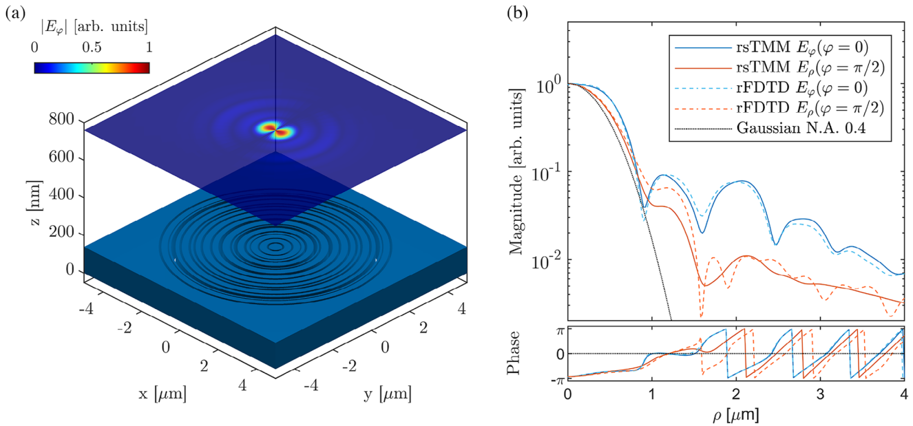
Figure 5. a Emission profile (top) achieved with a) bullseye structure (bottom), as optimized and simulated using rsTMM. b) Radial field profiles comparing results from rsTMM and rFDTD against the target Gaussian mode. The emission into the targeted Gaussian with N.A. = 0.4 is 42.44%, the overlap between rFDTD and rsTMM 98%.
