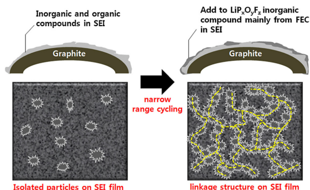
Fig. 6 Illustration of the effect of performing formation cycles within a narrow voltage range at low SOC with a FEC containing electrolyte on the SEI on graphite negative electrode. Reproduced with permission from Lee, 150 Elsevier, Copyright 2014.
