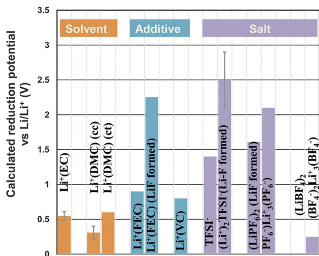
Fig. 27 Reduction potentials of electrolyte components according to the first principal simulation. Reprinted with permission from Wang et al. , 453 Springer Nature, Copyright 2018, who compiled the data of Delp et al. 459
