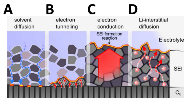
Fig. 28 Schematic of considered leakage mechanisms to reaction site enabling SEI growth. Reprinted with permission from Single et al. , 479 John Wiley and Sons, Copyright 2018.
