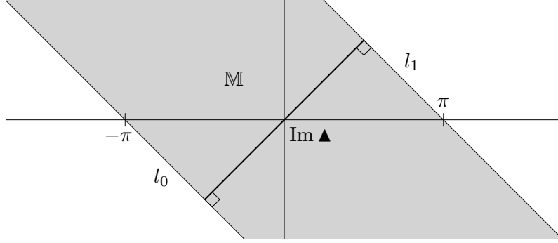
Figure 1.3: The strip \mathbb{M}_f and the image of the embedding \blacktriangle: \overline{\mathbb{R}} \rightarrow \mathbb{M}_f .
