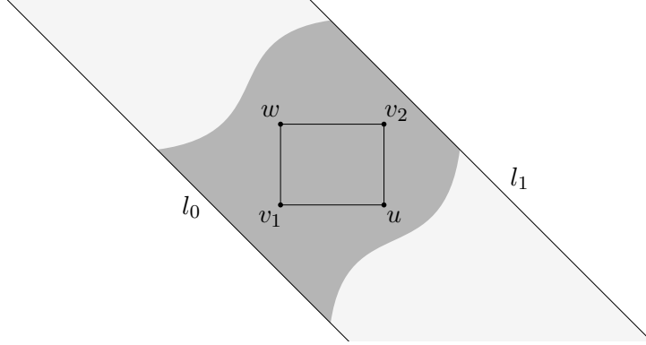
Figure 1.8: An axis-aligned rectangle u \preceq v_1, v_2 \preceq w \in D contained in the fundamental domain D , which is shaded in grey.
