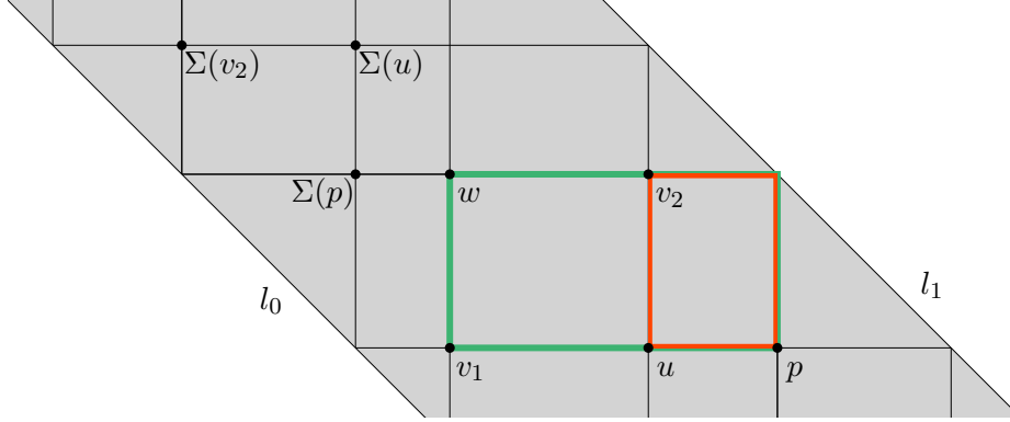
Figure 1.10: Axis-aligned rectangles determined by u , v_1 , v_2 , and w .
