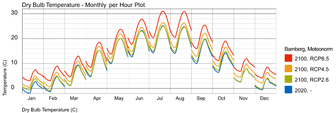
Figure 18 Comparison of the contemporary and future-updated weather files from Meteonorm for three various future scenarios - Dry Bulb Temperature
