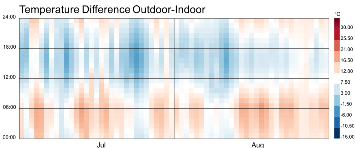
Figure 50 Temperature difference between indoor and outdoor conditions in the best-performing variant of the building in IC3 indicator
