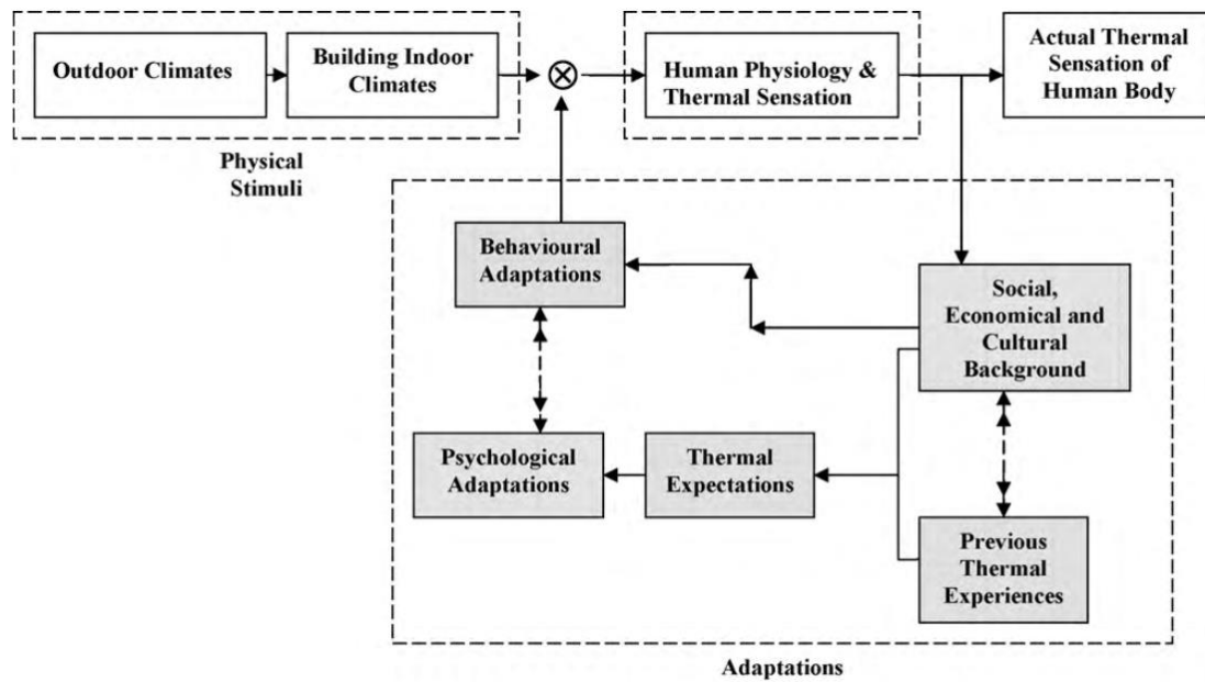
Fig. 2. The thermal comfort adaptive model mechanism.
