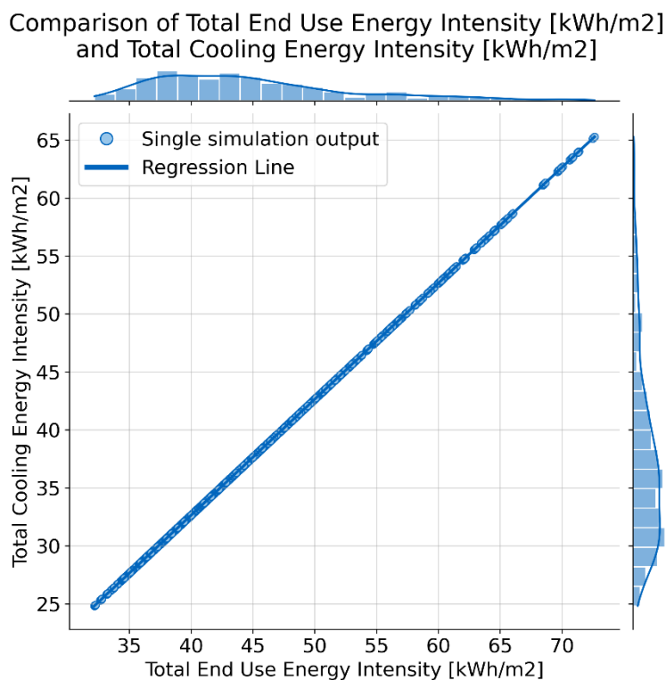
Figure 37 Scattered plot of the results of the simulation and a linear regression model
