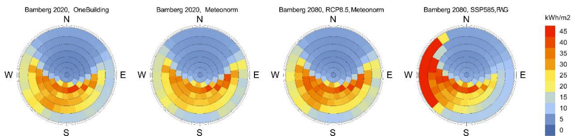
Figure 16 Comparison of contemporary and future-updated weather files - total global radiation
